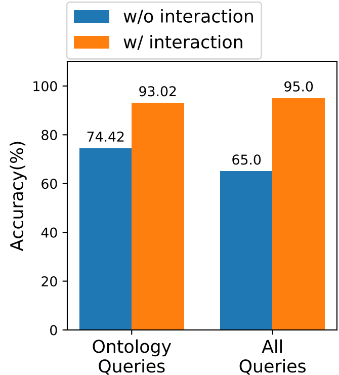
(a) Split Accuracy
