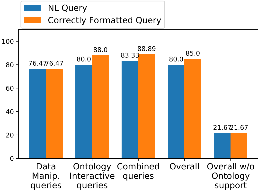
(b) Synthesis Accuracy
