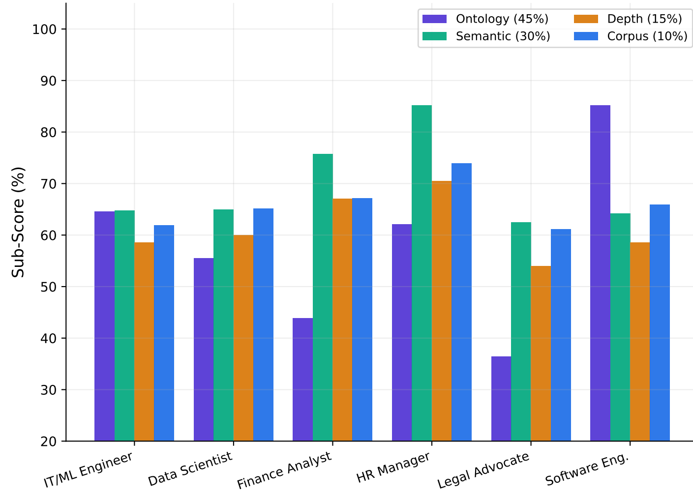
Fig. 3a Score Component Breakdown by Role
