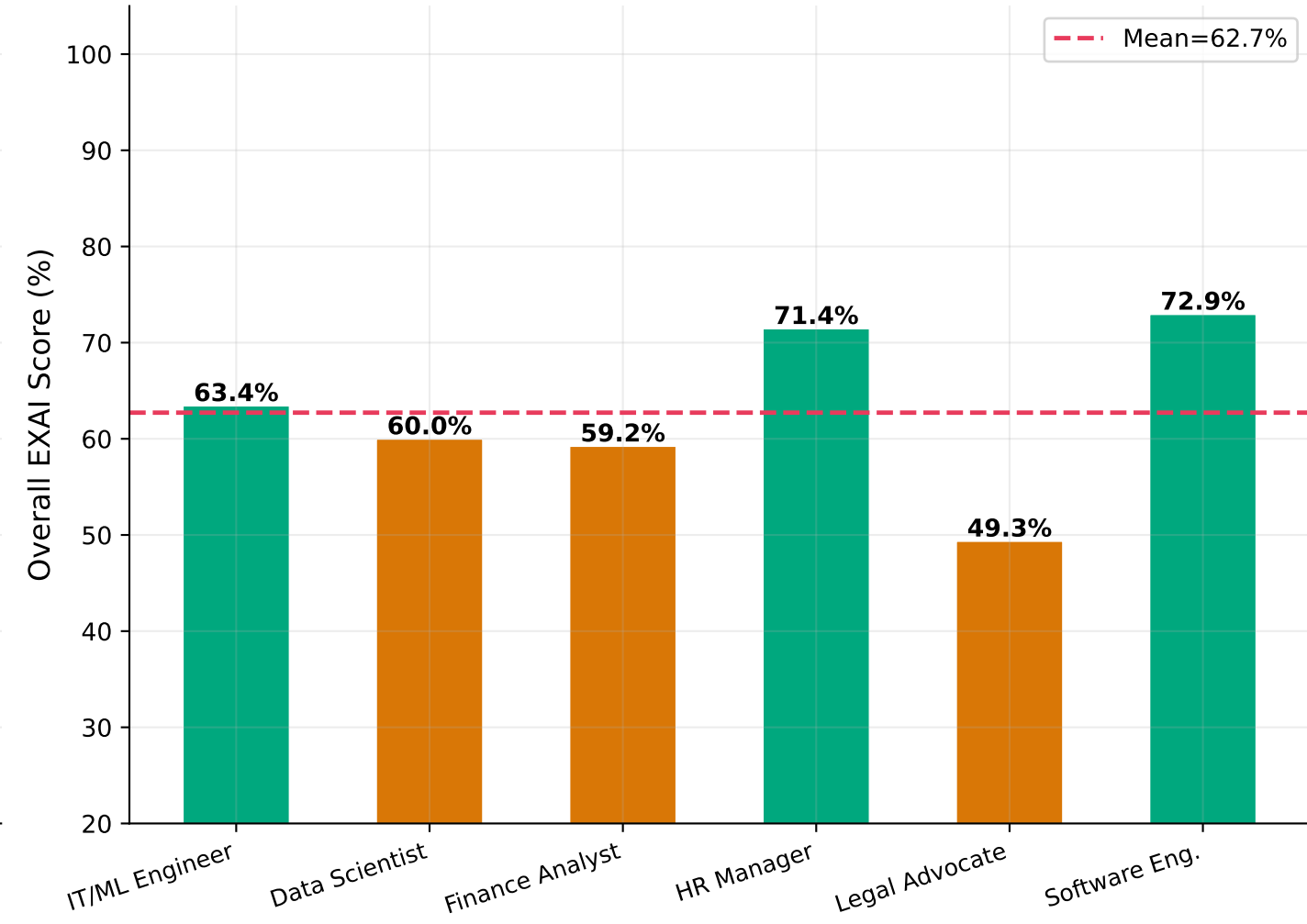
Fig. 3b Overall EXAI Score per Role
