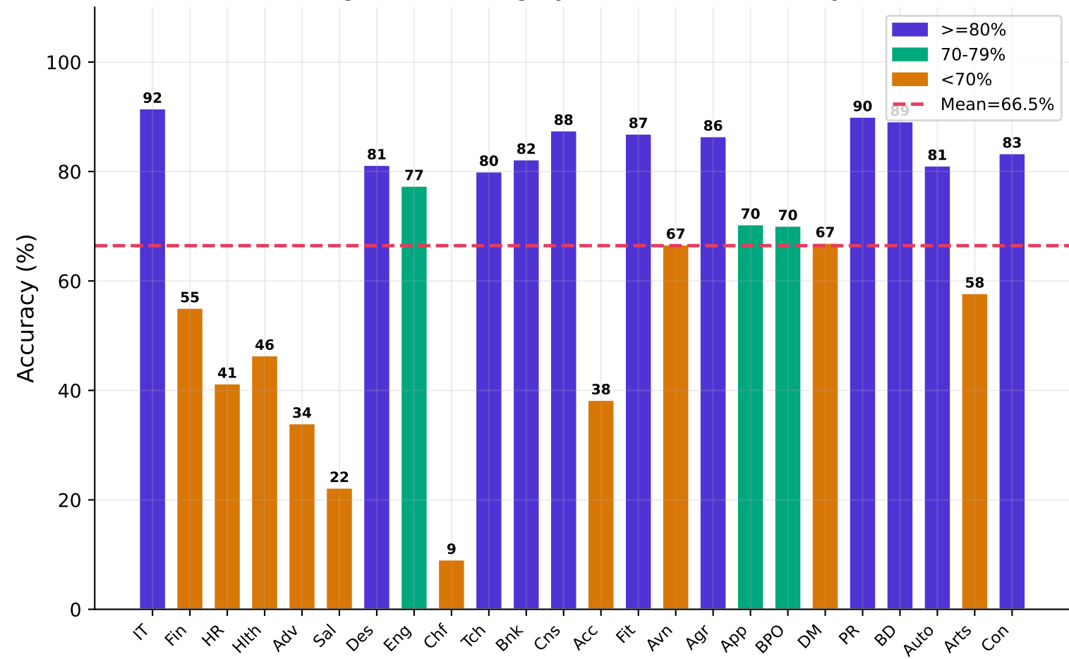
Fig. 4a Per-Category Classification Accuracy
