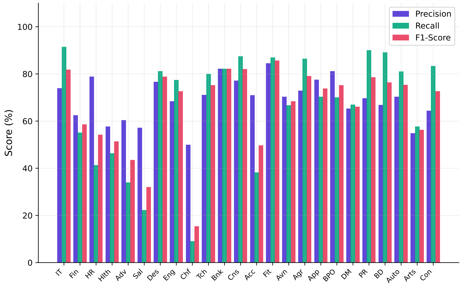
Fig. 4b Precision, Recall, F1 per Category (Macro: P=69.4% R=66.5% F1=66.0%)
