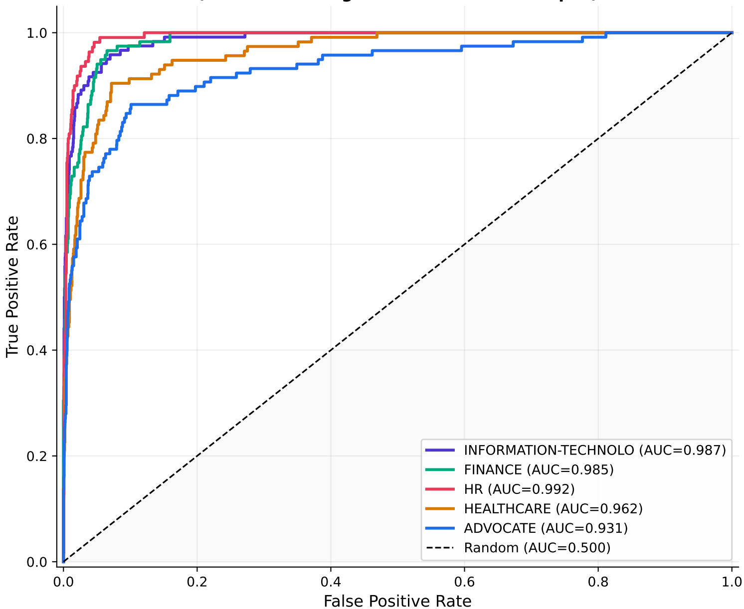
Fig. 5 ROC Curves — One-vs-Rest Classification (5 selected categories from 24-class corpus)
