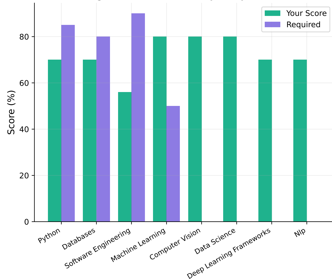
Fig. 6b Your Score vs Required per Skill
