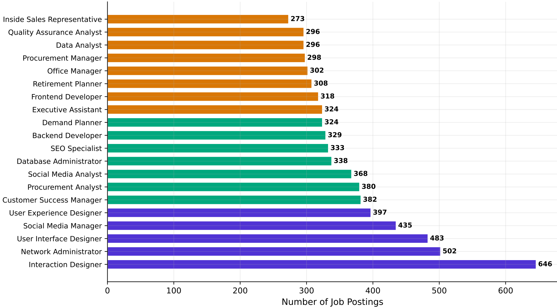
Fig. 9 Top-20 Job Roles — jobs_dataset_with_features.csv (50,000 rows sampled; total: 1,000,000+ postings)
