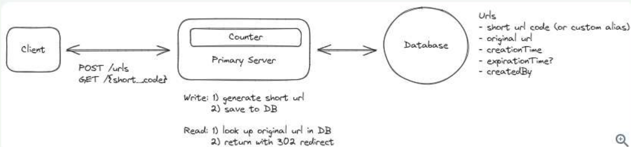
Unique Counter with Base62 Encoding
