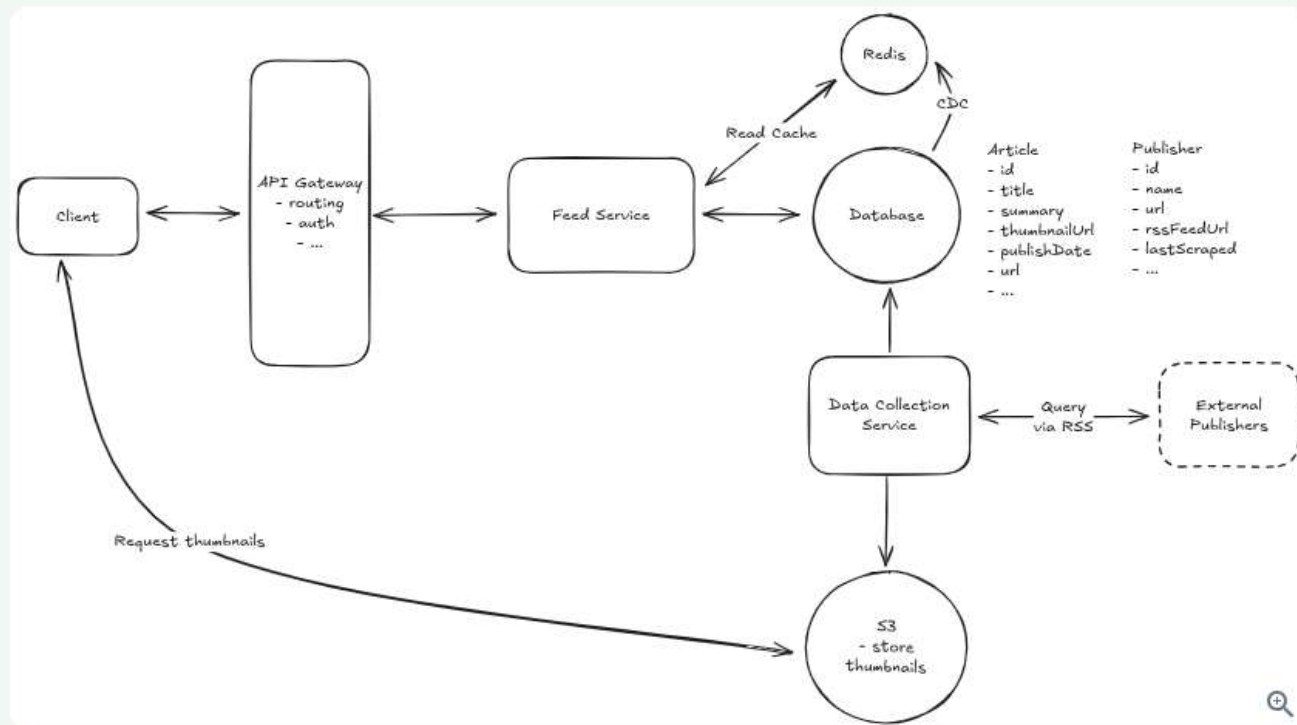
Real-time Cached Feeds with CDC
