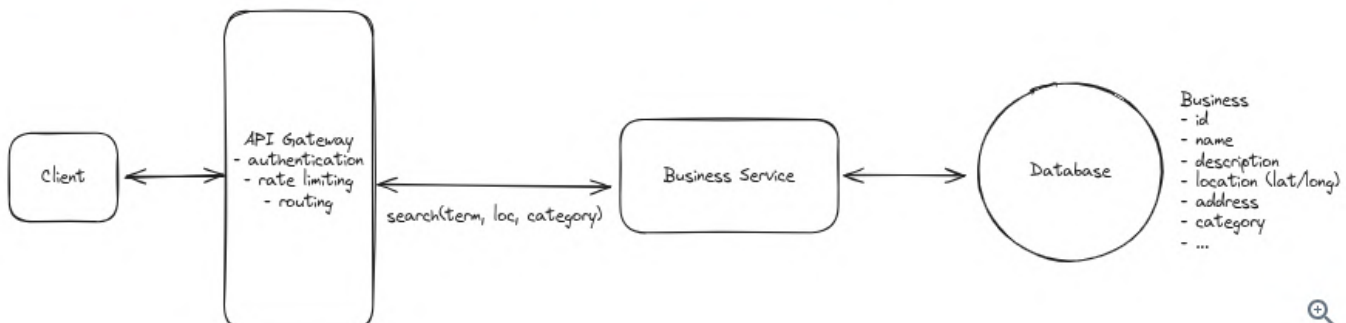
Yelp High-Level Design
