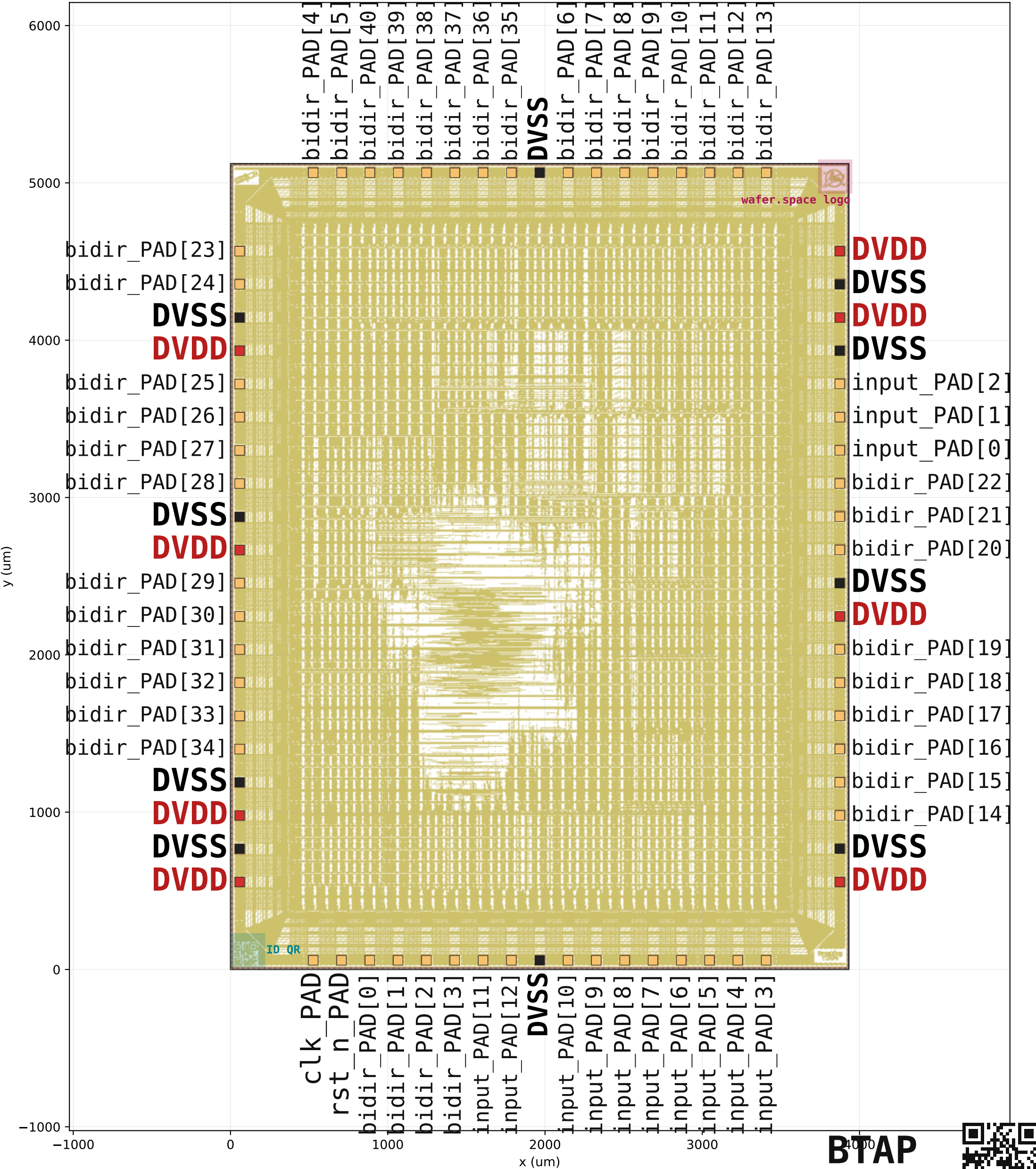
BTAP_chip_top_2_0 — 3932 x 5122 um — 74 labelled pads, 0 unlabelled
