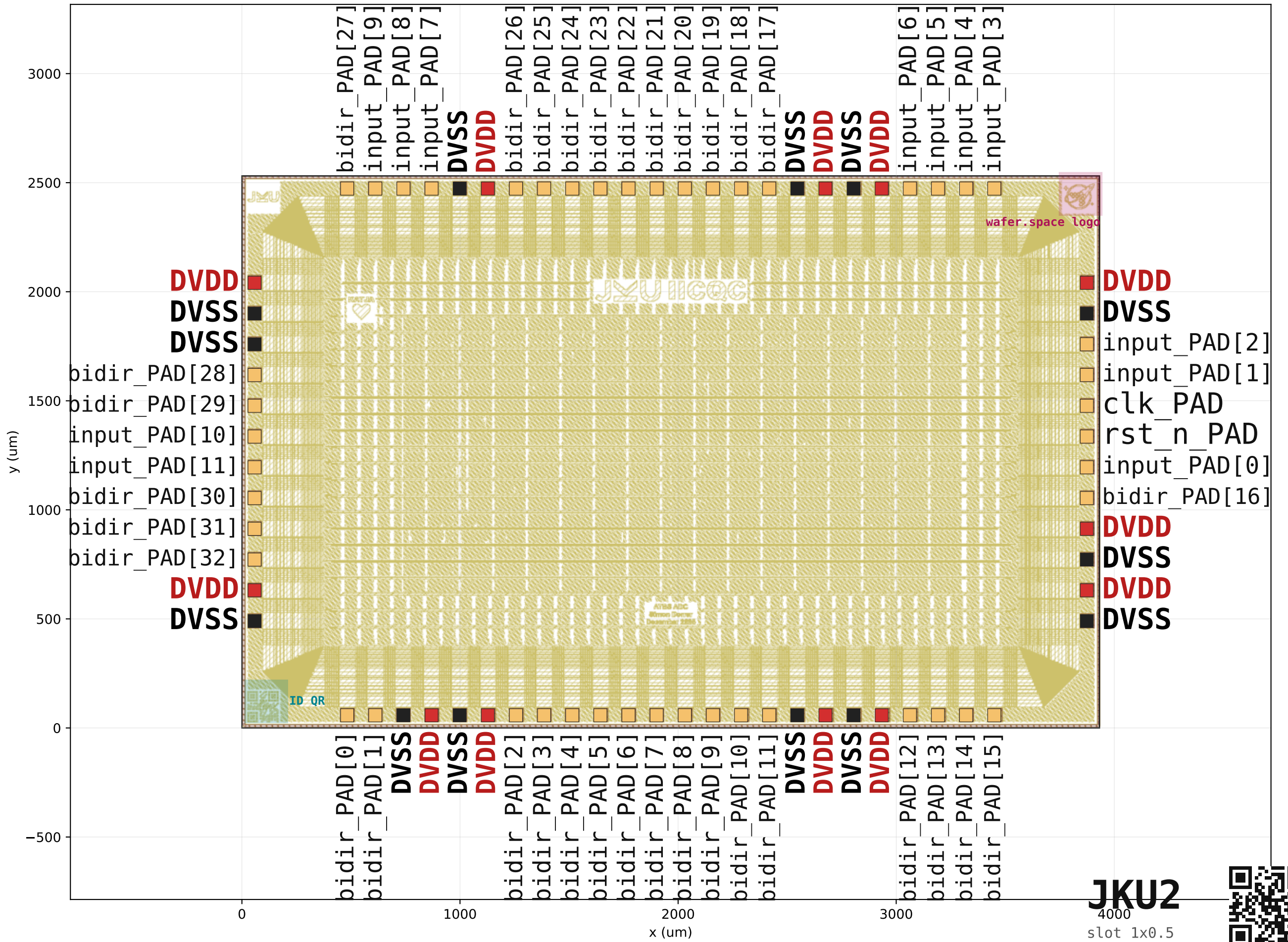
JKU2_chip_top_0_8 — 3932 x 2531 um — 72 labelled pads, 0 unlabelled
