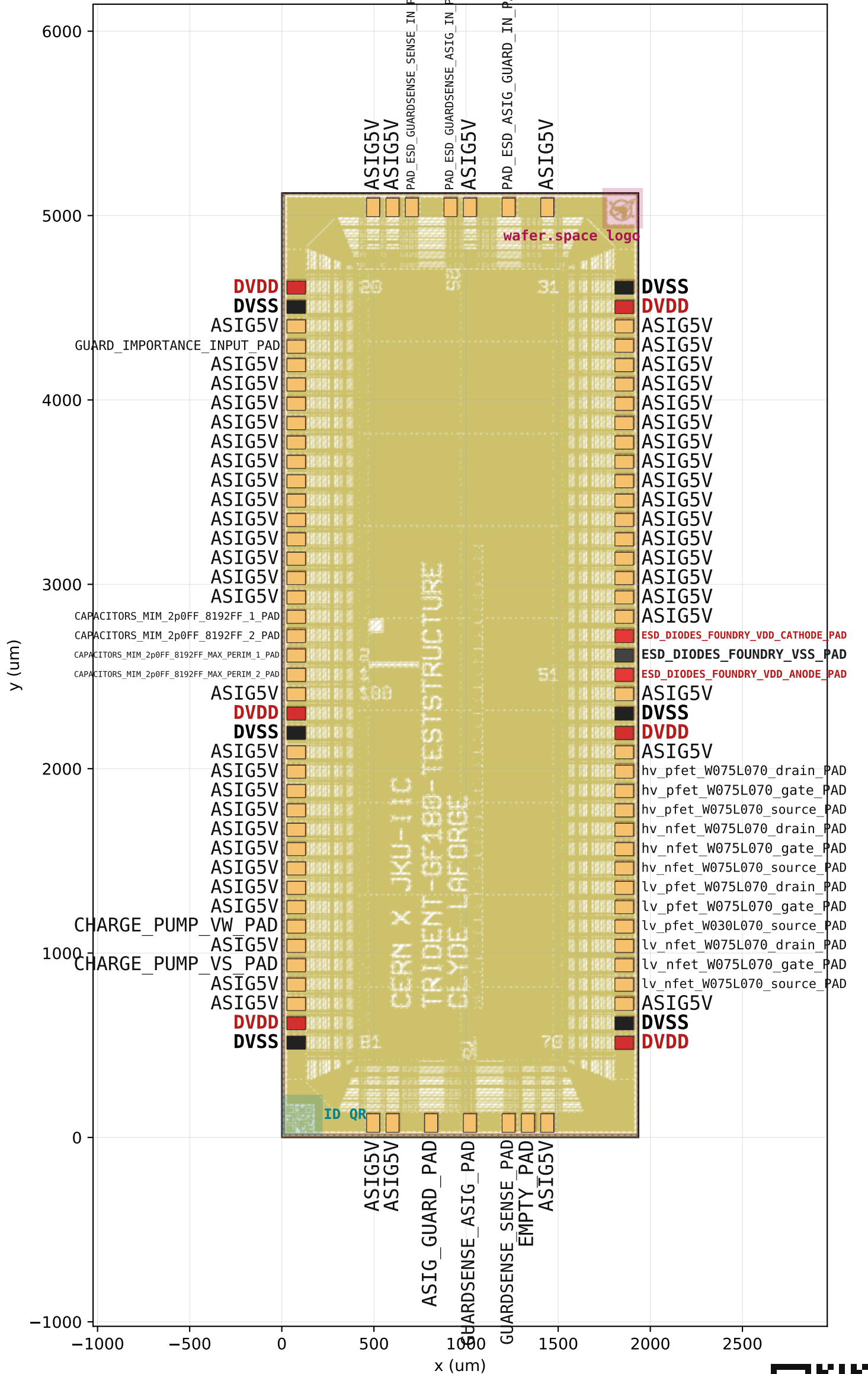
TRID_TOP_14_2 — 1936 x 5122 μm — 94 labelled pads, 0 unlabelled
