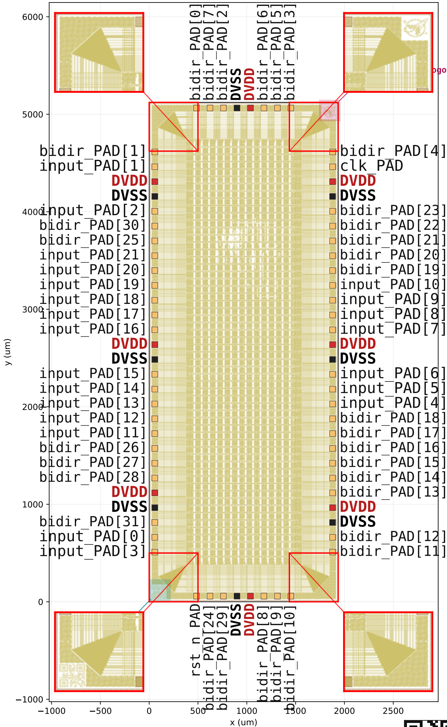
HZ80_chip_top_14_0 — 1936 x 5122 um — 72 labelled pads, 0 unlabelled
