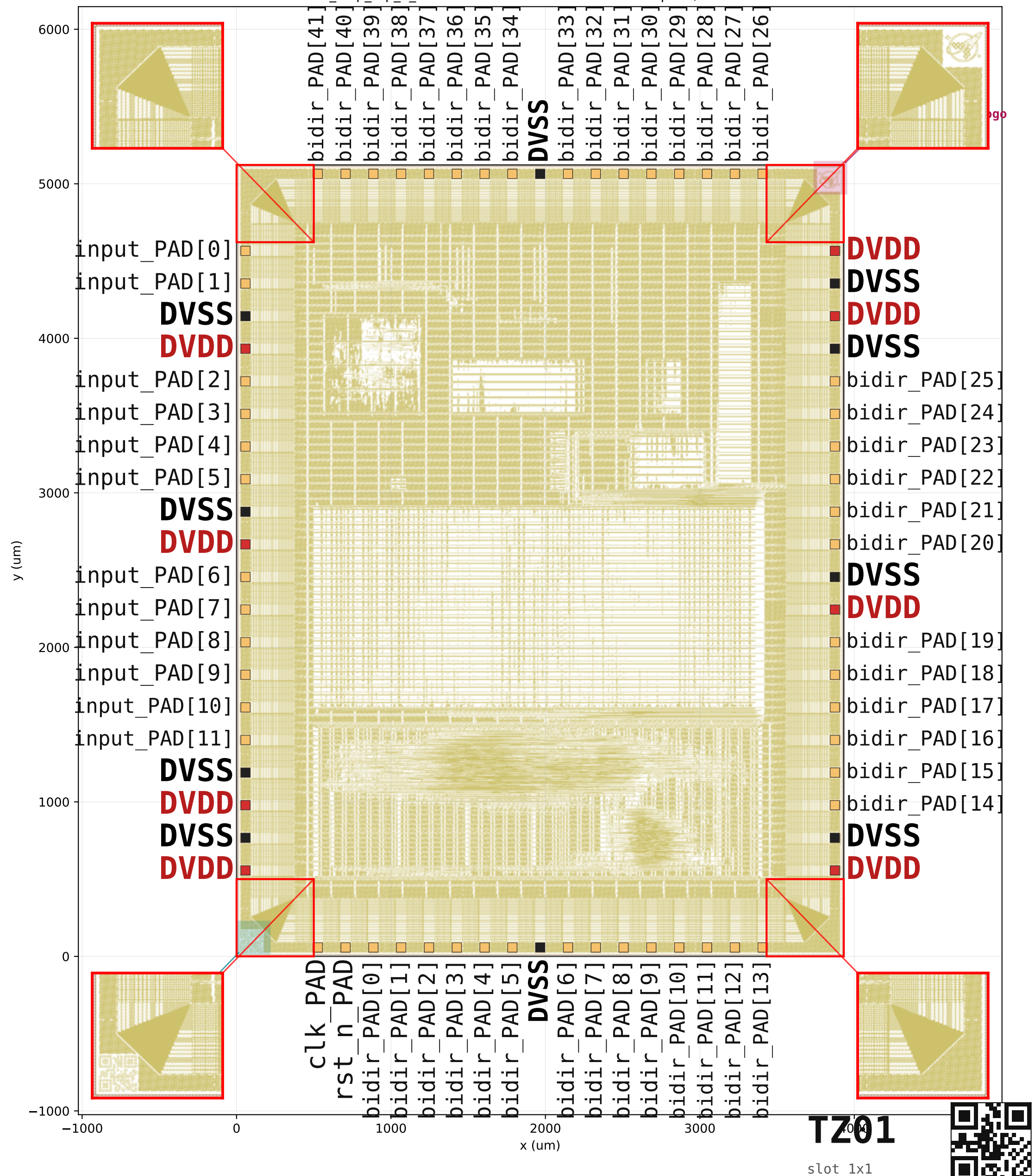
TZ01 chip top 0 4 — 3932 x 5122 um — 74 labelled pads, 0 unlabelled
