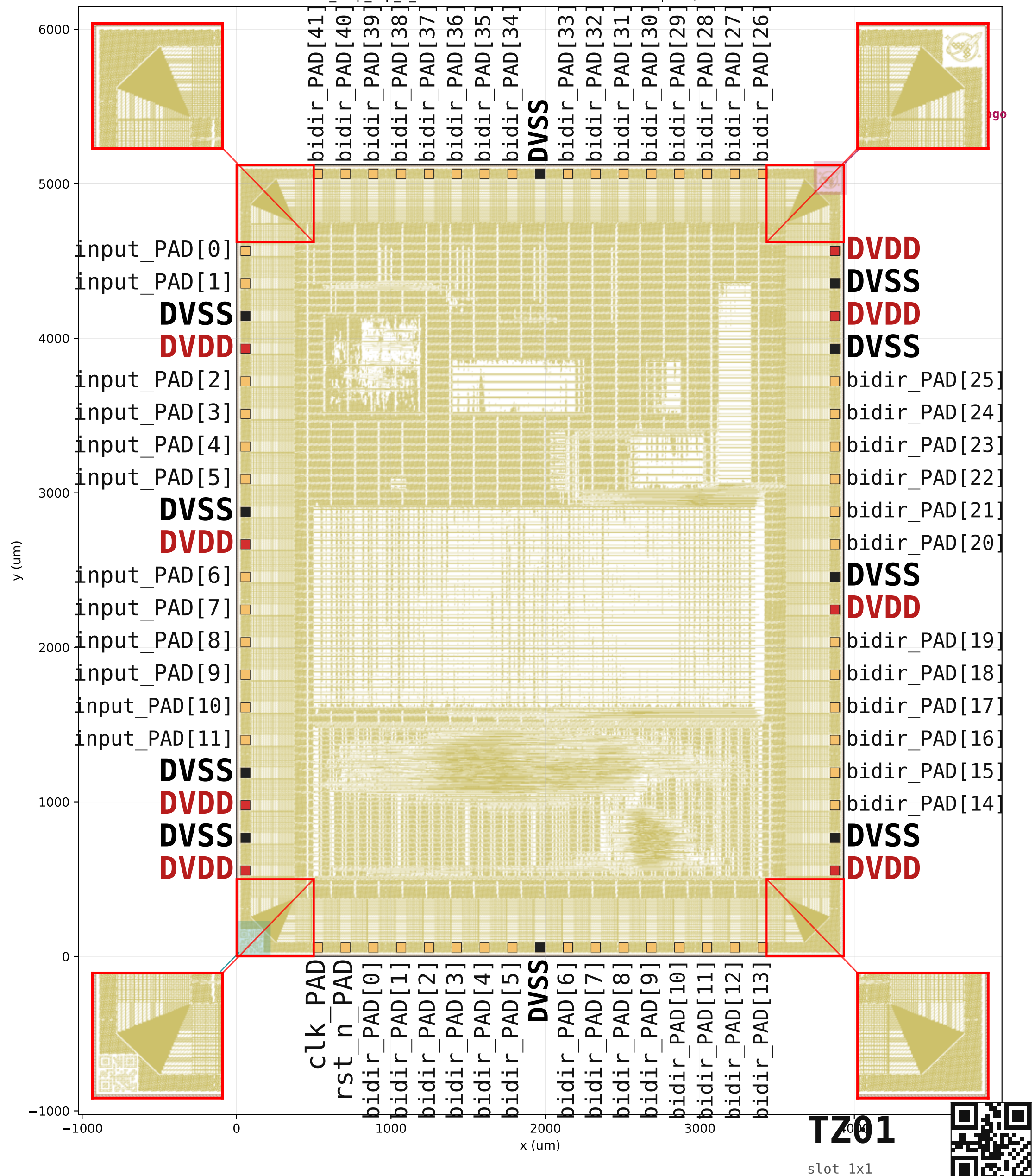
TZ01 chip top 2 4 — 3932 x 5122 um — 74 labelled pads, 0 unlabelled
