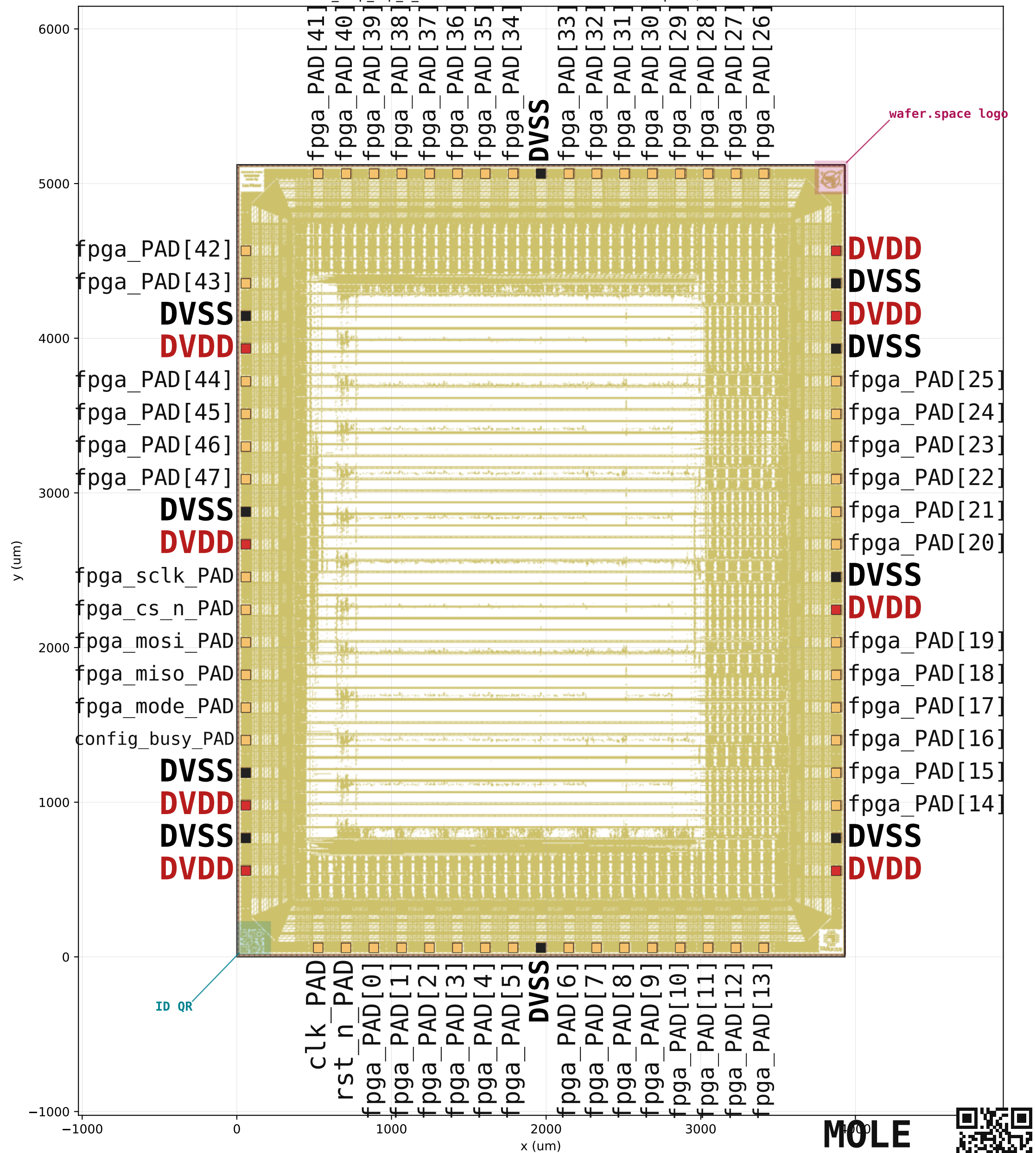
MOLE chip top 8 4 — 3932 x 5122 um — 74 labelled pads, 0 unlabelled
