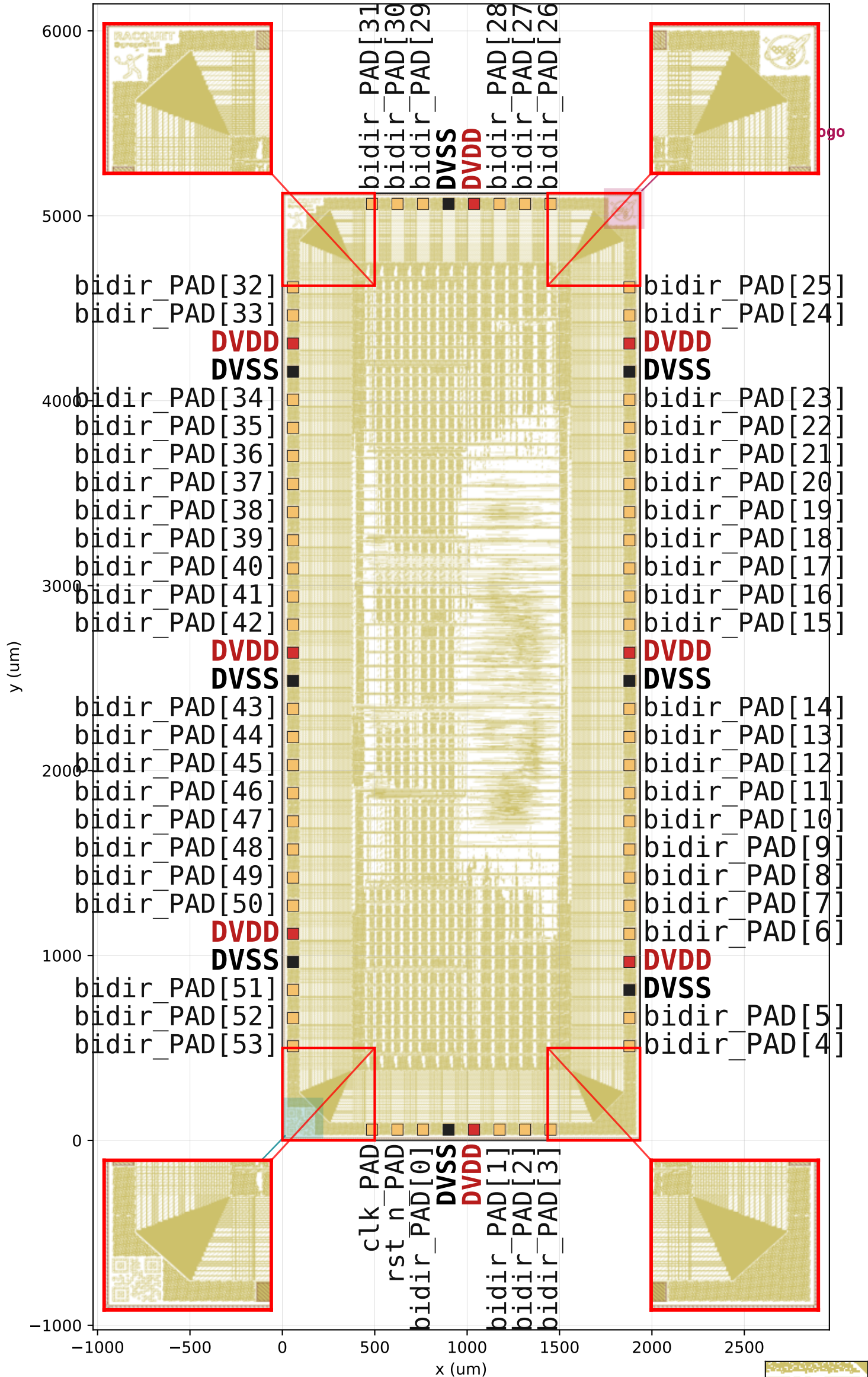
GD02_chip_top_14_4 — 1936 x 5122 um, 72 labelled pads, 0 unlabelled
