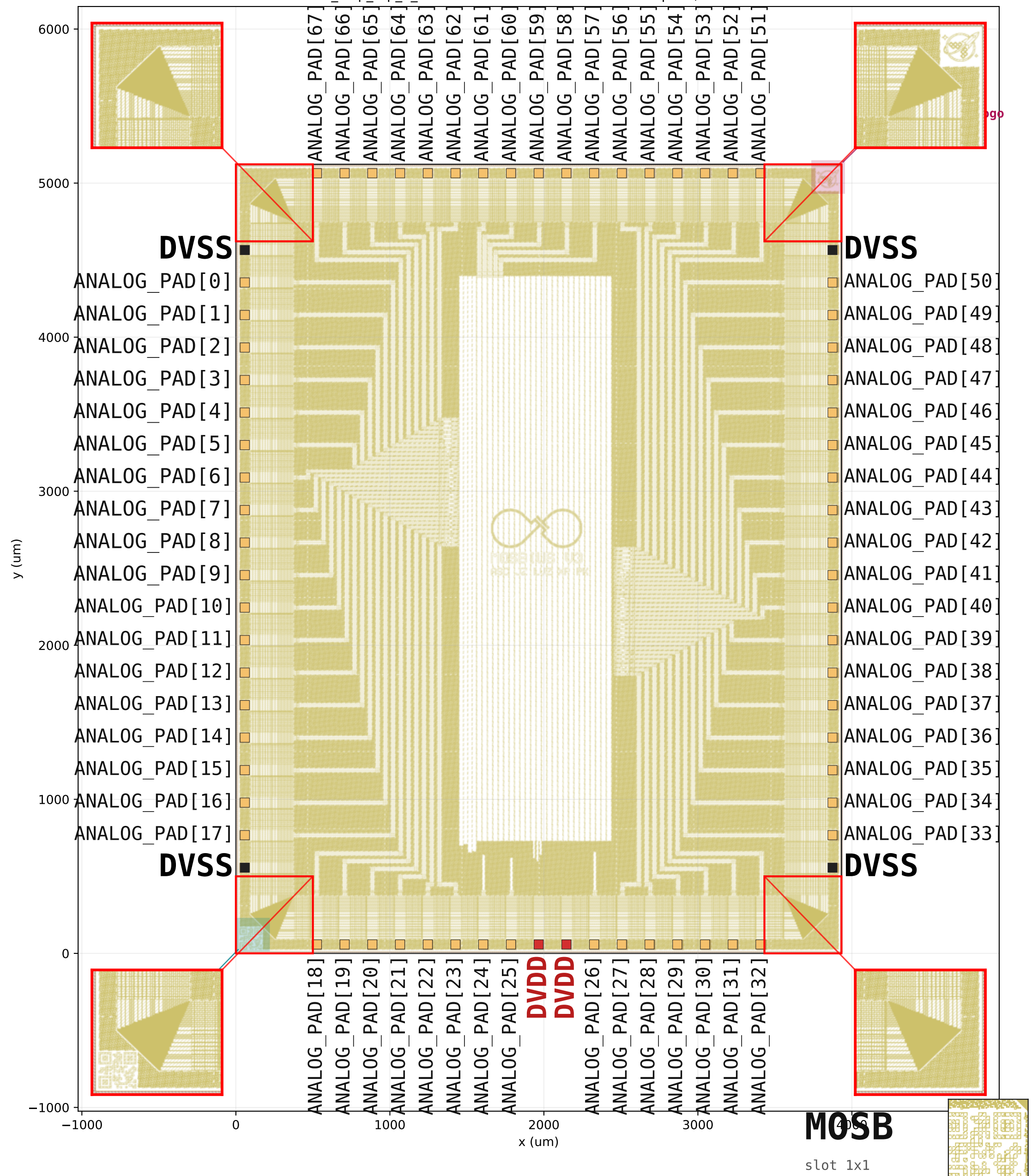
MOSB_chip_top_4_2 — 3932 x 5122 um — 74 labelled pads, 0 unlabelled
