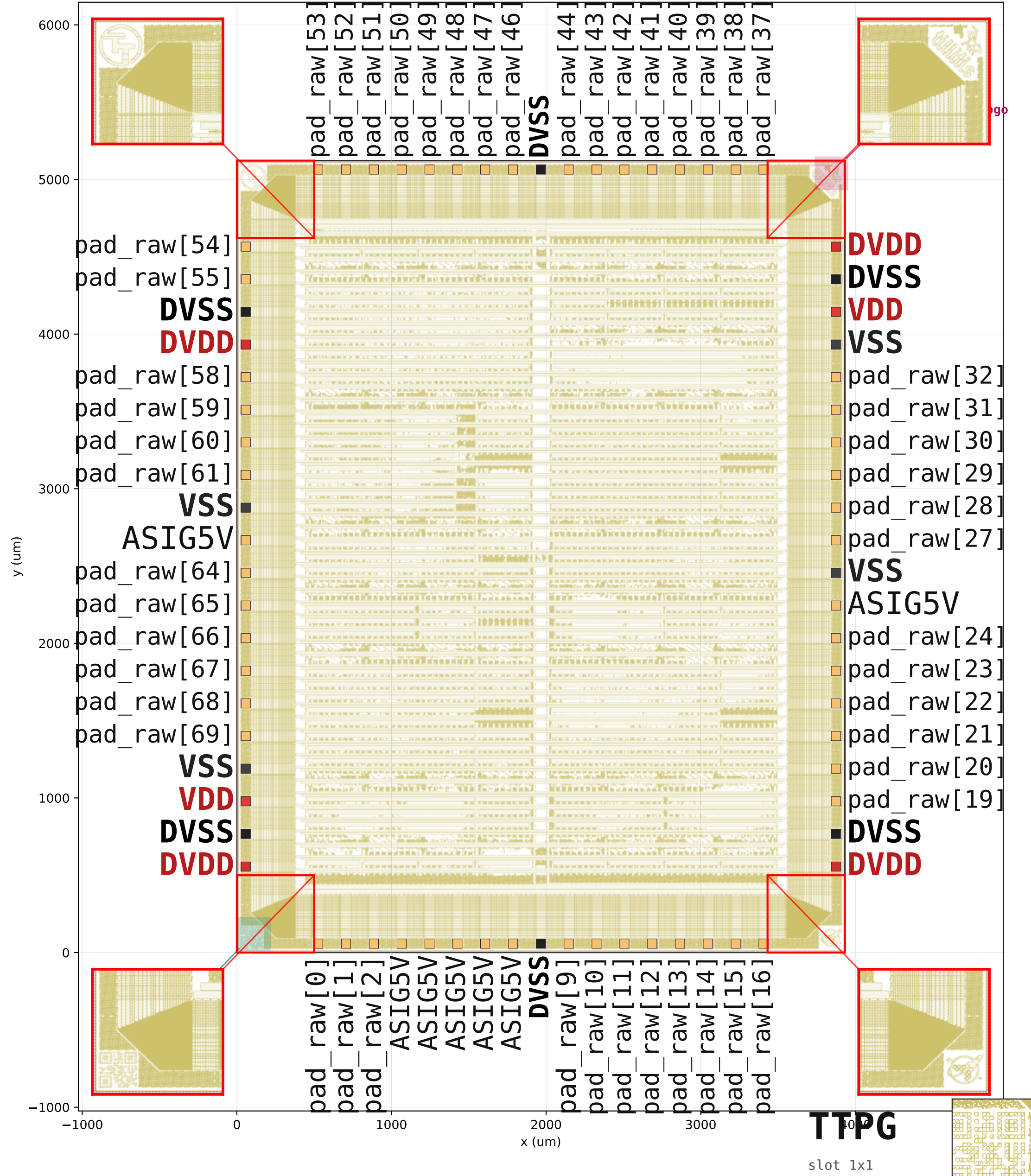
TTPG_tt_gf_wrapper_6_2 — 3932 x 5122 um — 74 labelled pads, 0 unlabelled
