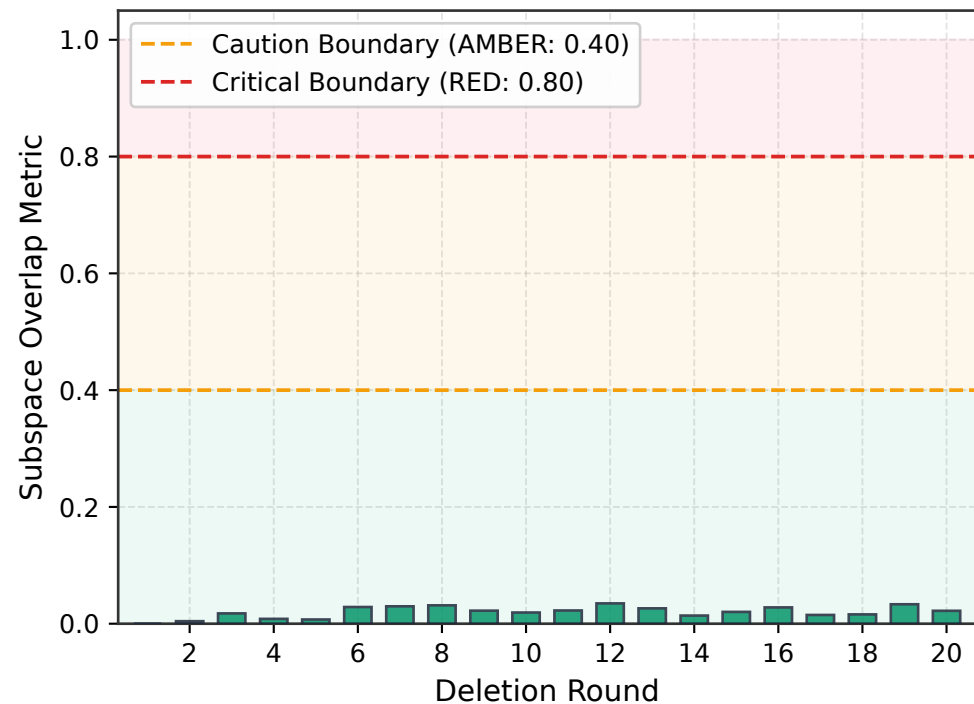
(a) SOM Subspace Overlap Score \|Q_k^T g_t\|/\|g_t\|
