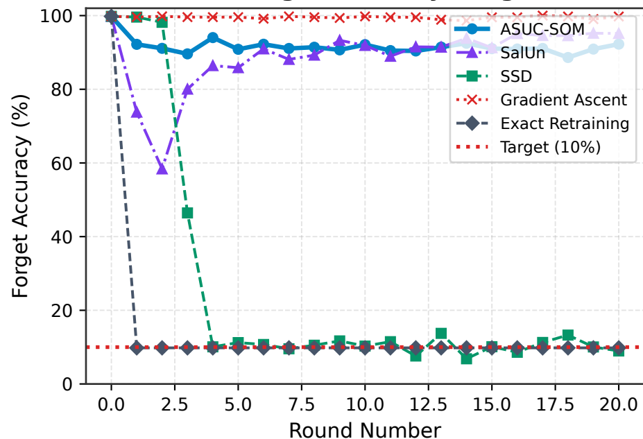
(b) Residual Forget Accuracy (Target \leq 10\% )
