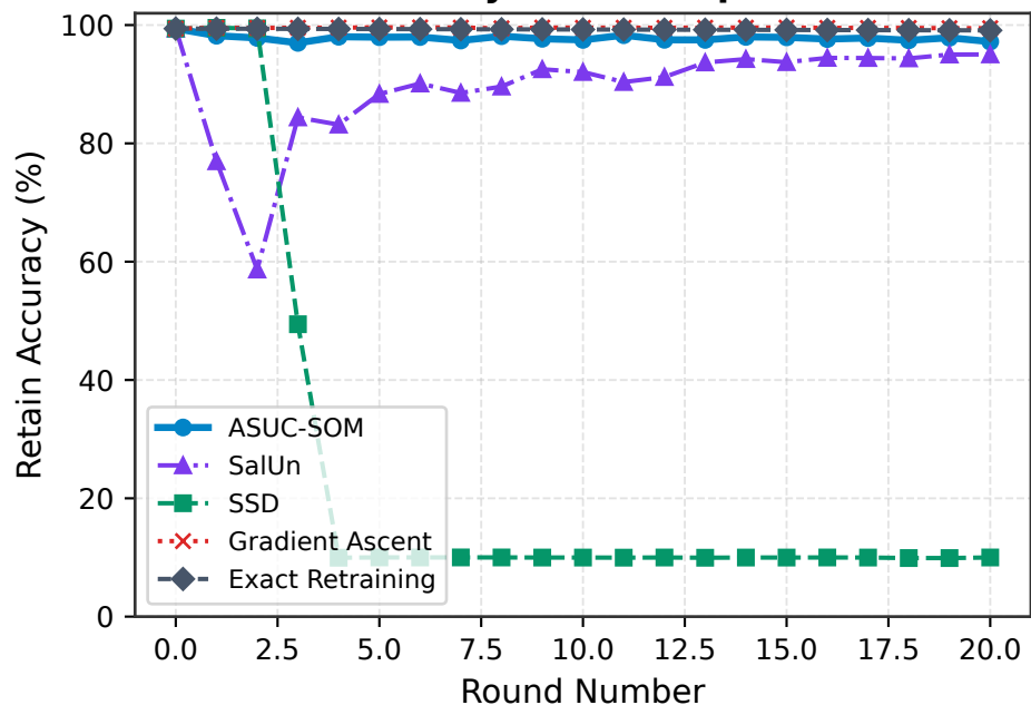
(a) Retain Accuracy Under Sequential Deletion
