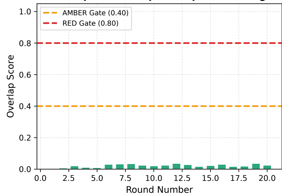
(c) SOM Subspace Overlap & Adaptive Routing Trigger
