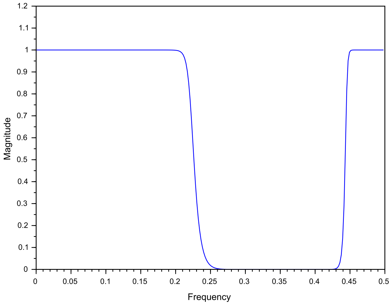
Butterworth IIR Band Stop Filter
