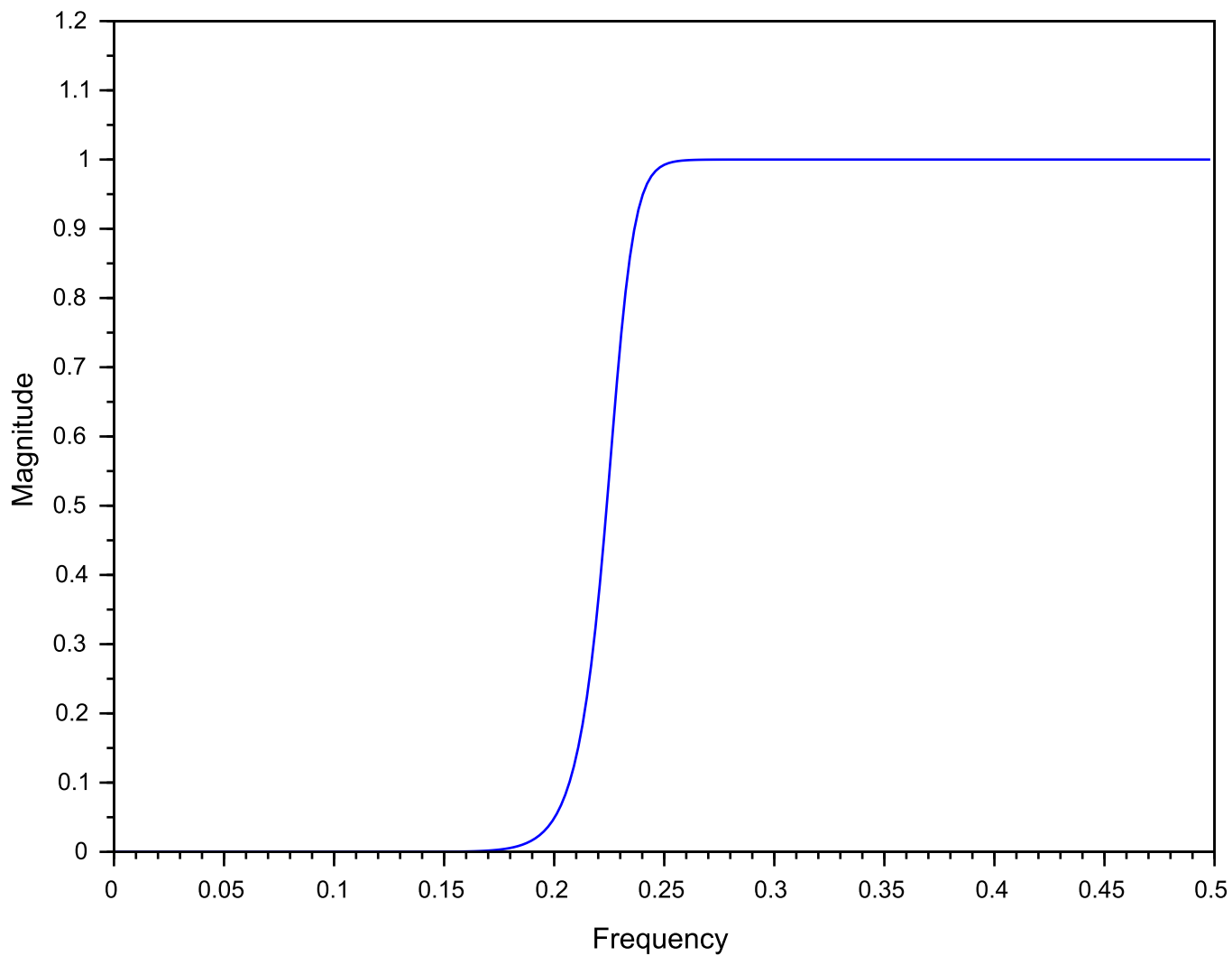
Butterworth IIR High Pass Filter
