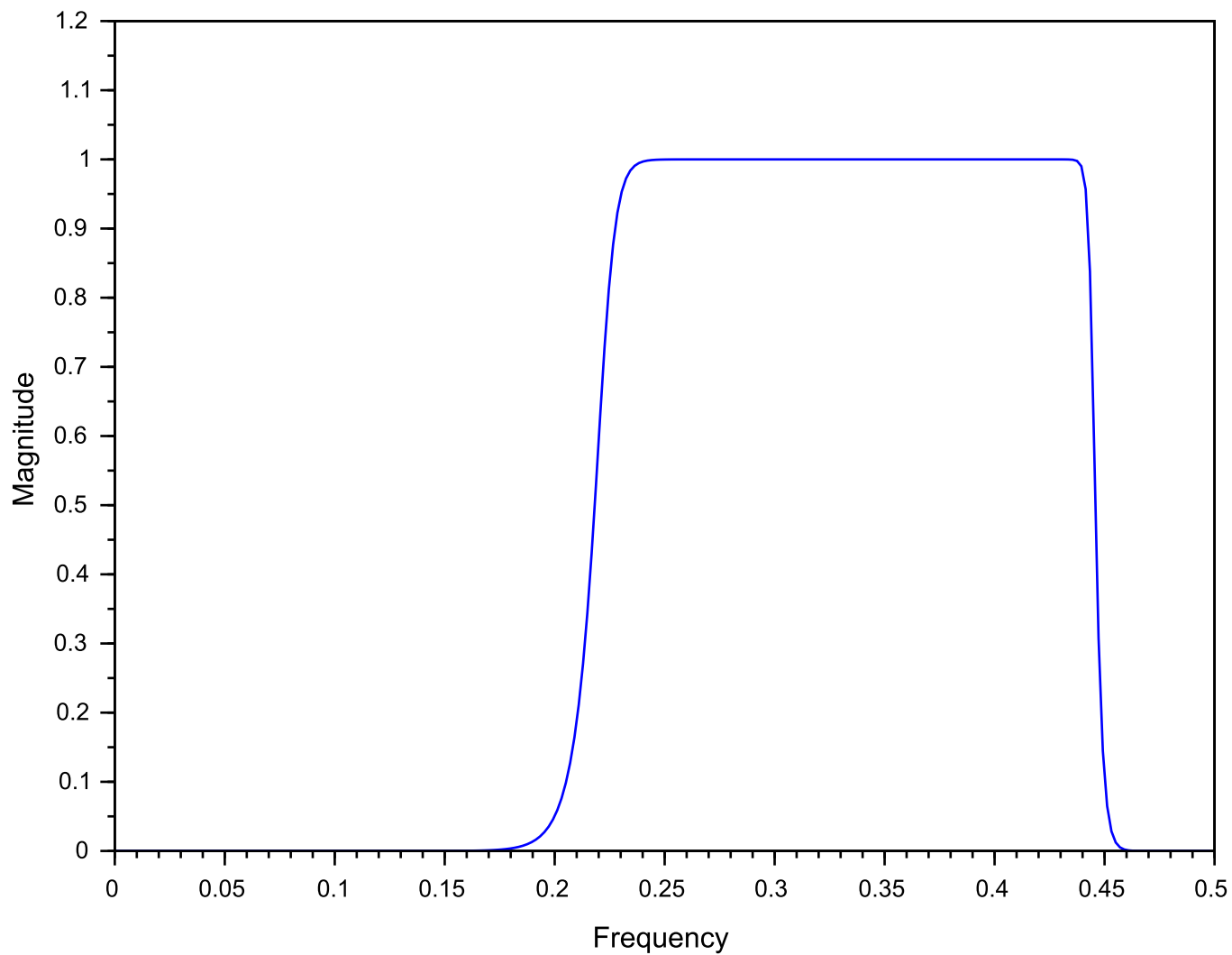
Butterworth IIR Band Pass Filter
