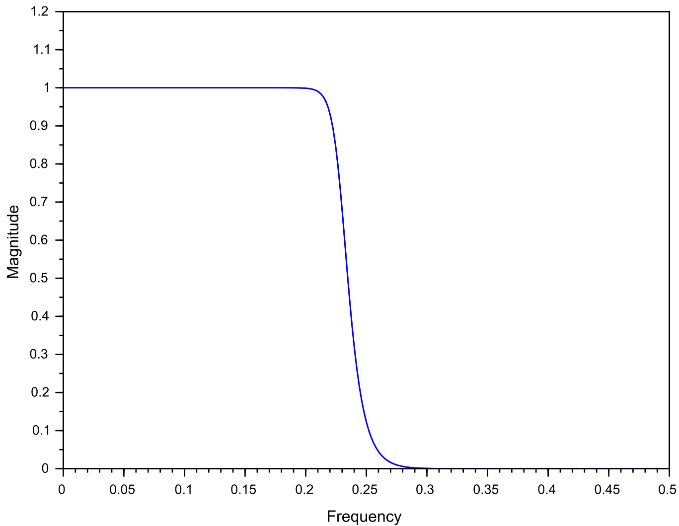
Butterworth IIR Low Pass Filter
