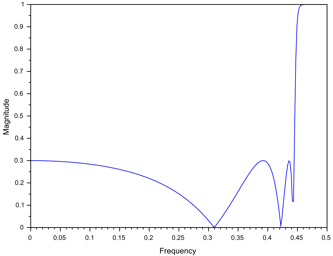
Chebyshev IIR HIGH PASS Filter
