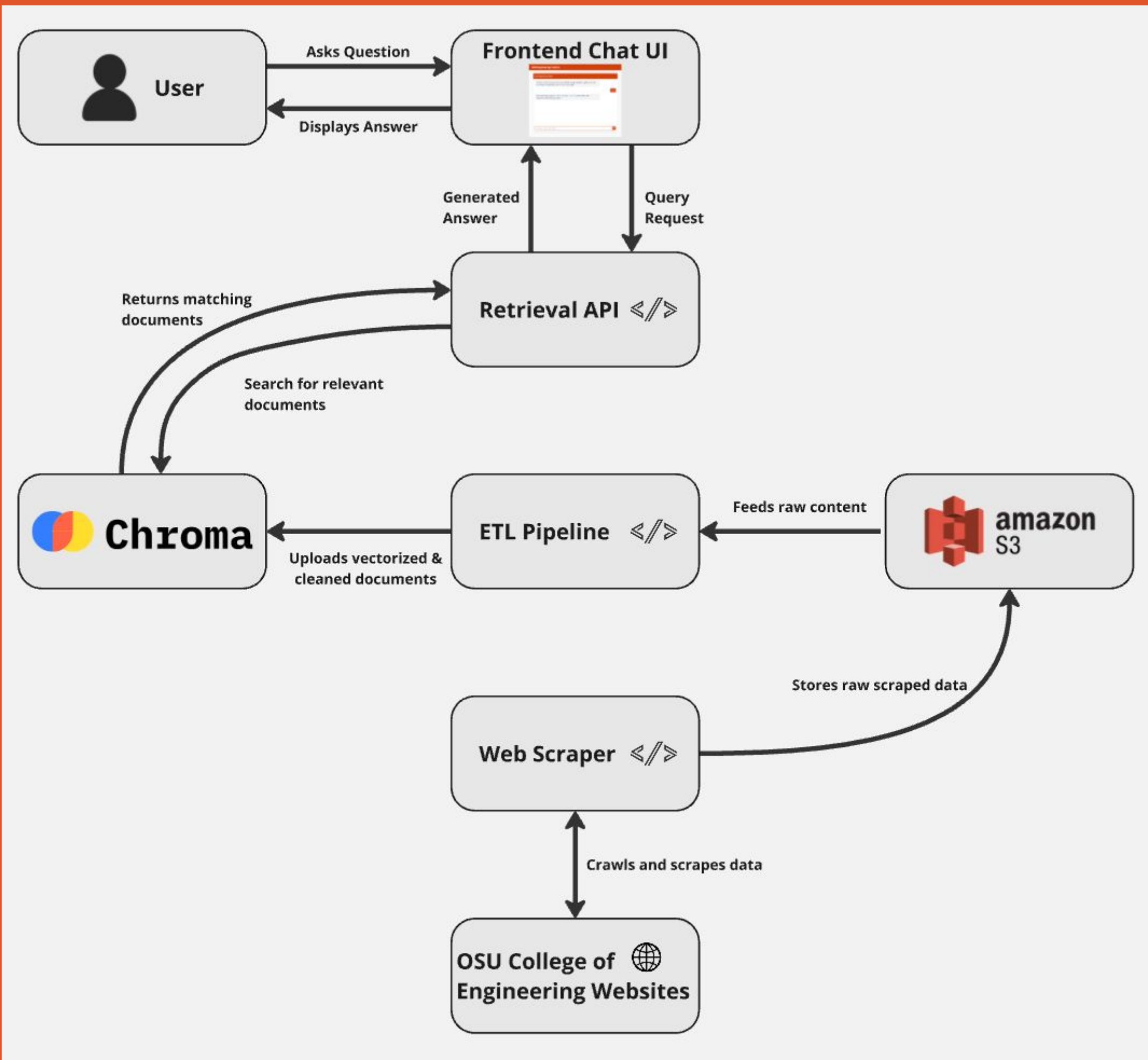
Figure 1: High-level overview of our system architecture
