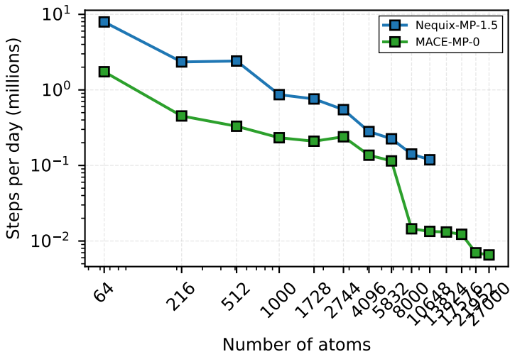
Benchmark NVIDIA H100 PCIe float32
