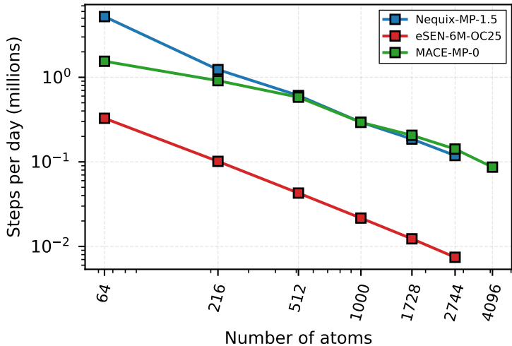
Benchmark Tesla T4 float32
