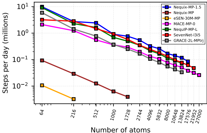
Matbench compliant, Si diamond lattice_constant=5.43 Å NVIDIA A100-SXM4-80GB float32
