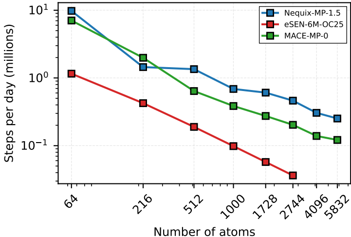
Benchmark NVIDIA A100-SXM4-80GB float32
