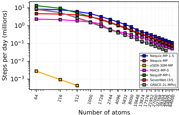
Matbench compliant, Si diamond lattice_constant=5.43 Å NVIDIA H100 80GB HBM3 float32
