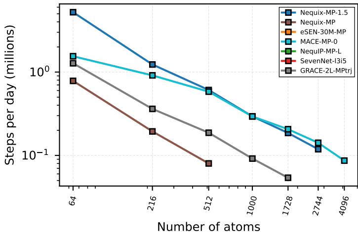
Matbench compliant, C diamond a=3.567 \text{ \AA} Tesla T4 float32
