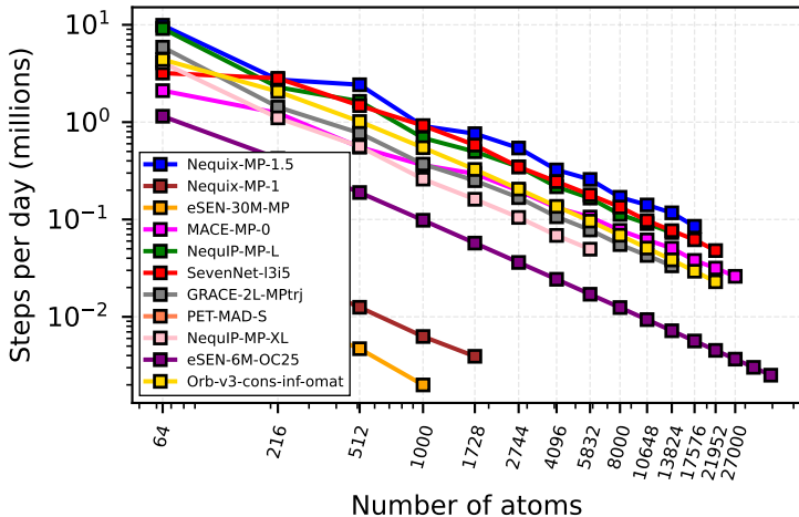
Matbench non-compliant, Si diamond lattice_constant=5.43 Å NVIDIA A100-SXM4-80GB float32
