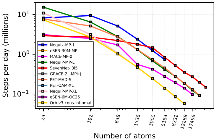
Matbench non-compliant, H2O.csv H2O Å NVIDIA H100 80GB HBM3 float32
