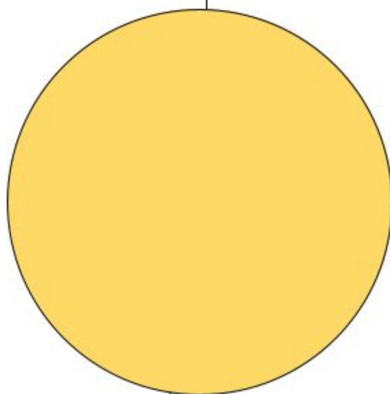
Saturn
