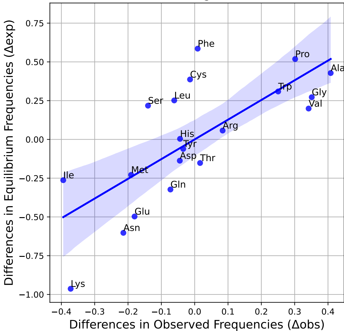
Including Cov
