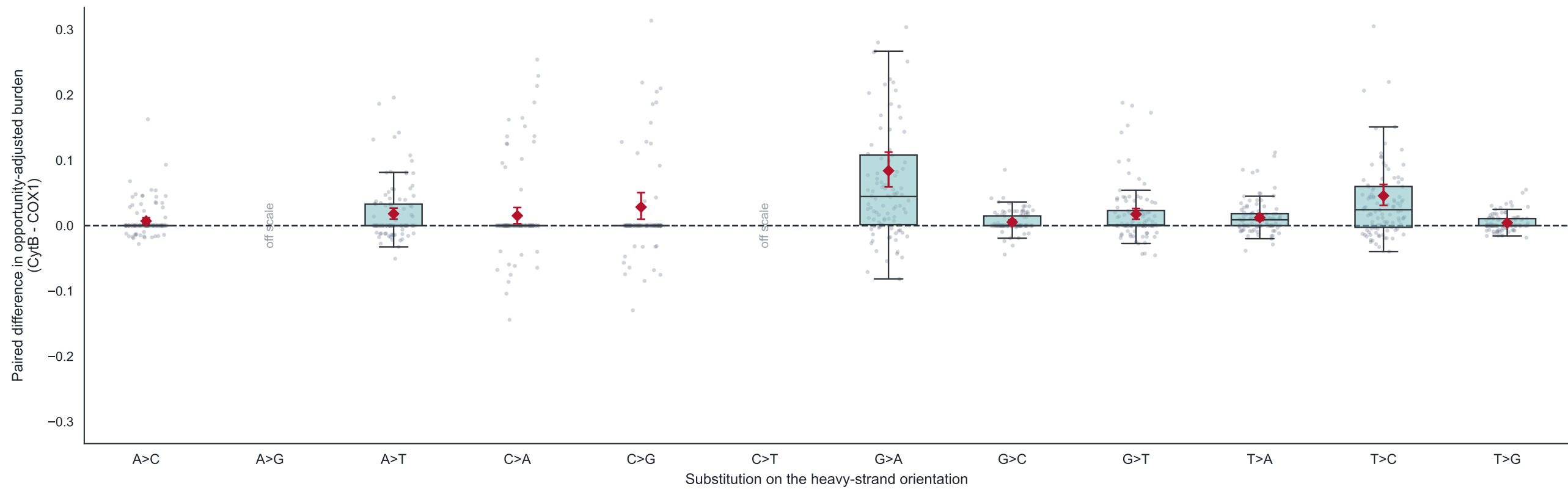
Same differences, scaled to the smaller components; A>G, C>T omitted here
