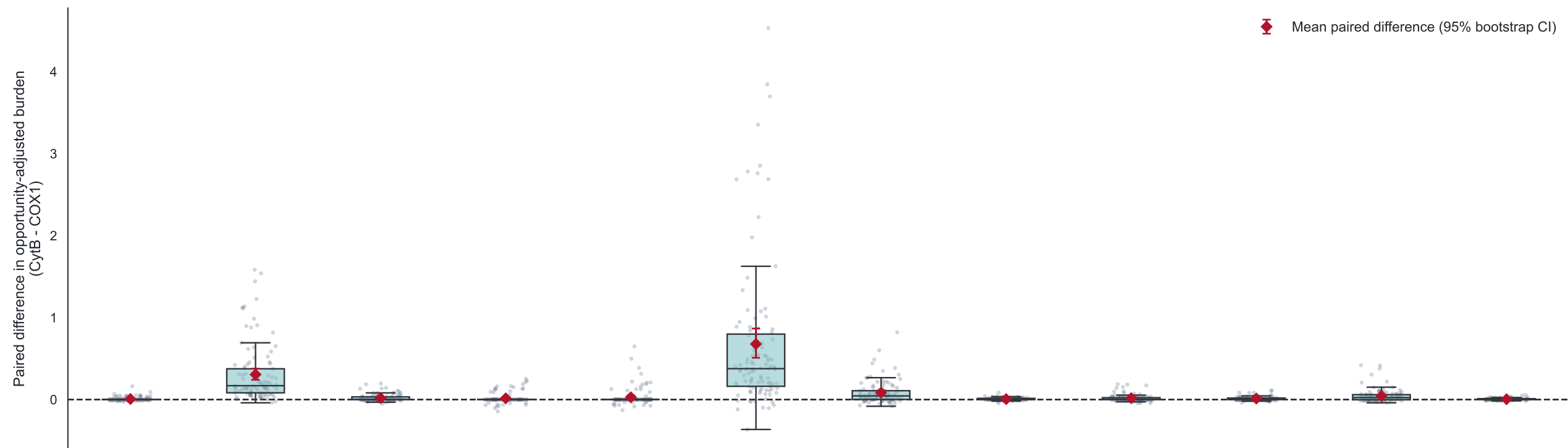
Same differences, scaled to the smaller components; A>G, C>T omitted here
