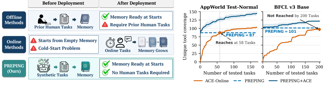
Figure 1: PREPING builds memory before the first user task and mitigates online cold-start. Left: Unlike offline methods that require prior human tasks or online methods that start from empty memory, PREPING constructs procedural memory through self-generated synthetic practice before deployment. Right: PREPING establishes broad tool coverage before deployment, whereas ACE-Online must accumulate coverage from user-facing tasks, requiring 58 tasks to match PREPING on AppWorld and still falling short after 200 tasks on BFCL v3.
