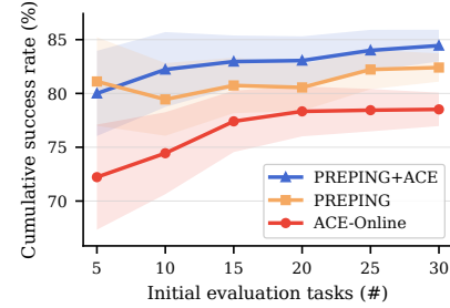
Figure 3: PREPING mitigates online cold-start before memory builds up.
