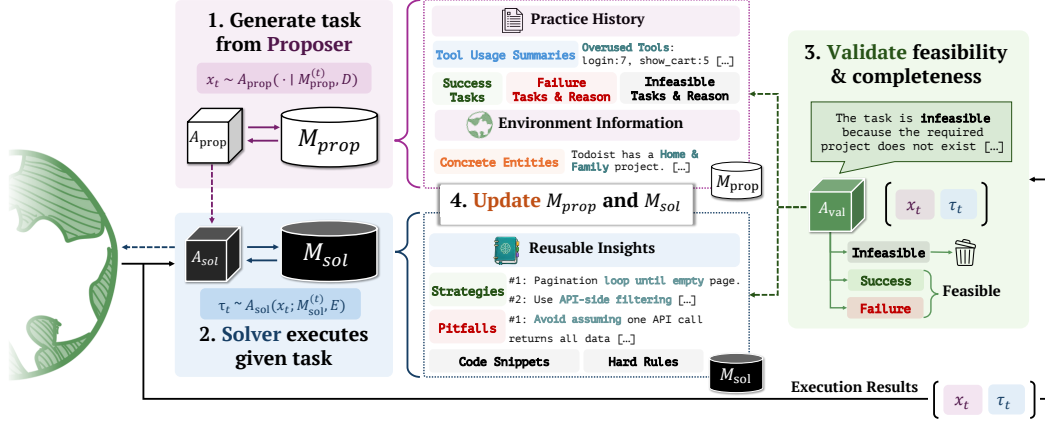
Figure 2: Overview of PREPING. PREPING builds procedural memory before deployment through a synthetic-practice loop: proposing tasks, executing them in the environment, validating the resulting trajectories, and updating memory. Proposer memory ( M_{\text{prop}} ) shapes what to practice next, while the Validator filters which synthetic trajectories are reliable enough to become solver memory ( M_{\text{sol}} ).
