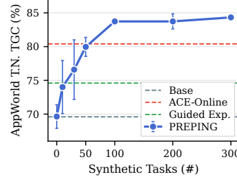
Figure 4: Construction budget. AppWorld Test-Normal TGC as a function of the number of synthetic tasks.
