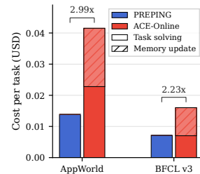
Figure 5: Deployment time cost per task.
