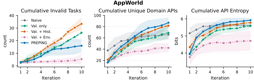
Figure 16: Iteration dynamics of AppWorld component ablations.
