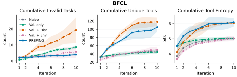
Figure 17: Iteration dynamics of BFCL component ablations.
