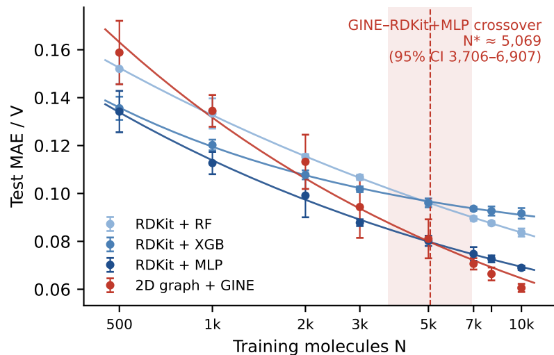
A Random split: power-law fits
