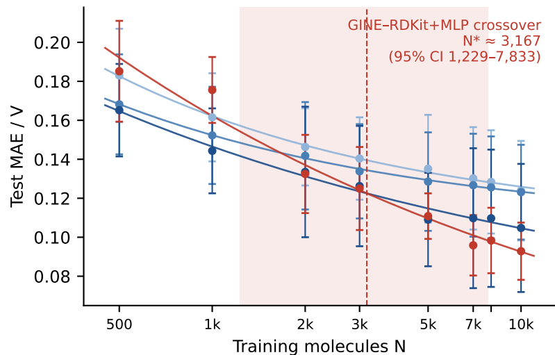
B Scaffold split: power-law fits
