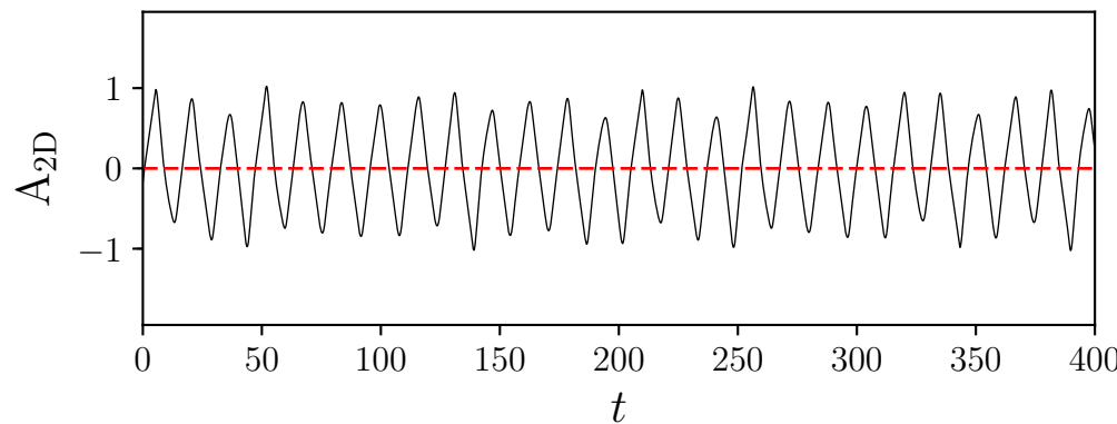
(a) Ra = 3 \cdot 10^5 inside i - ii
