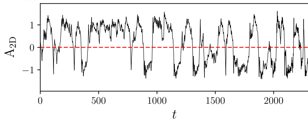
(c) Ra = 8 \cdot 10^6 inside ii - iii
