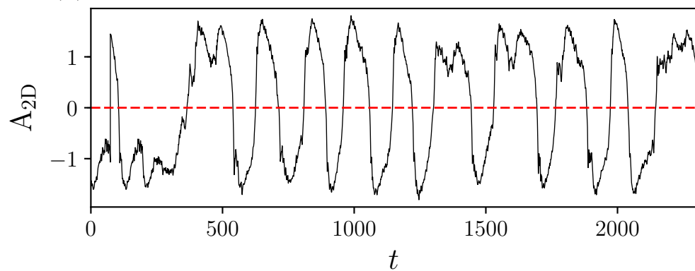
(e) Ra = 1 \cdot 10^8 inside iv - v
