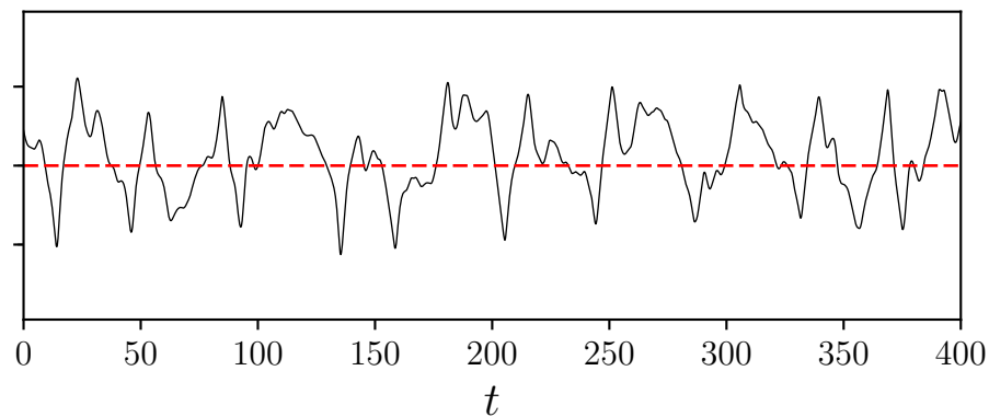
(b) Ra = 2 \cdot 10^6 inside i - ii
