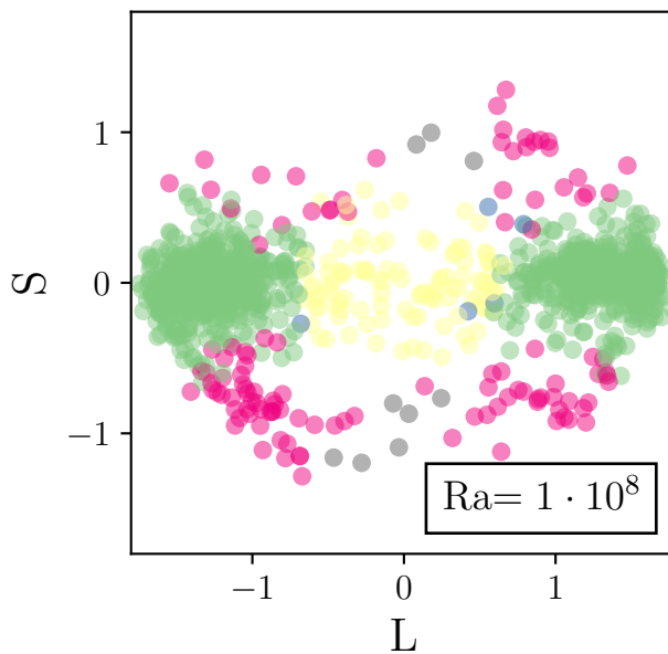
(e) Ra = 1 \cdot 10^8 inside iv - v
