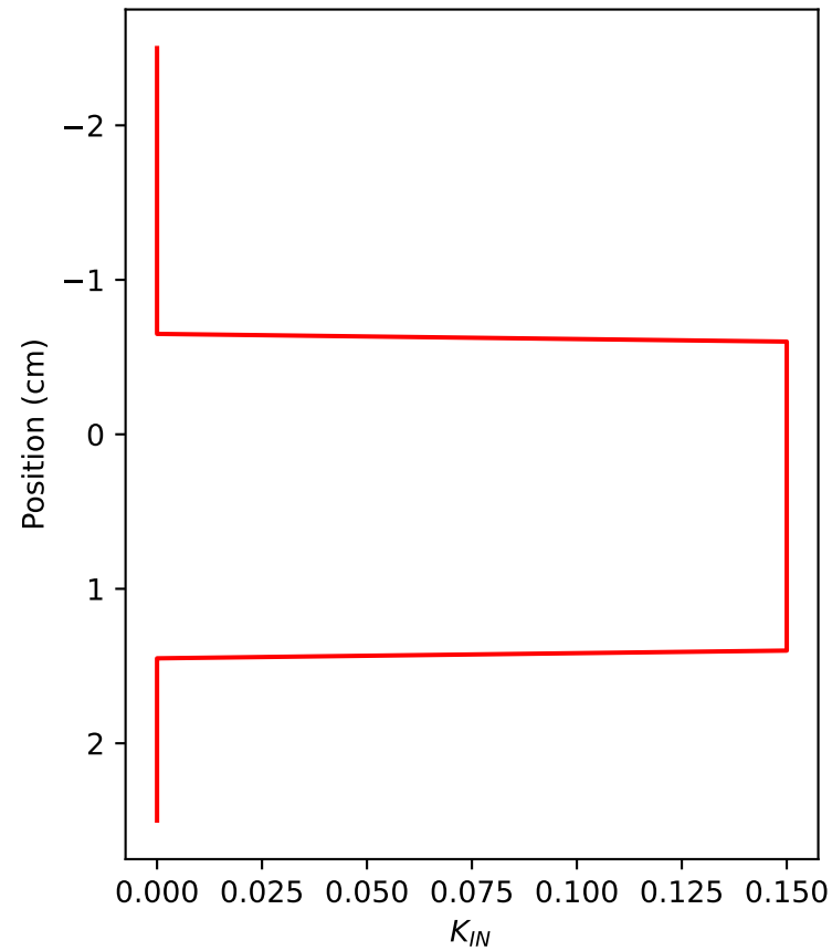
K_{IN} kernel
