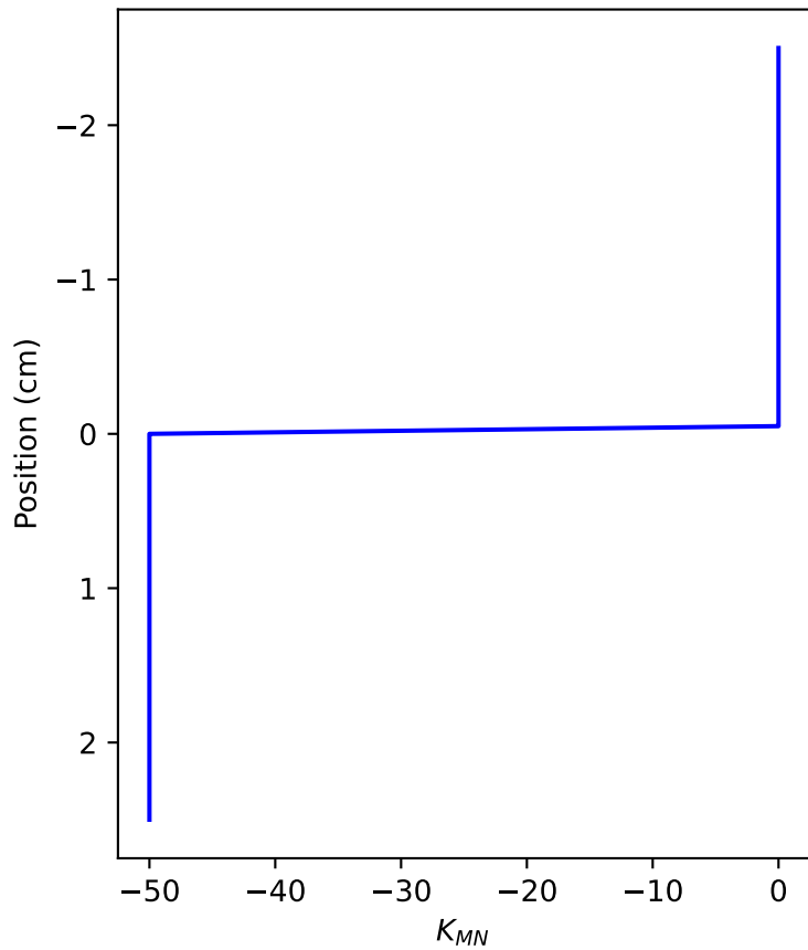
K_{MN} kernel
