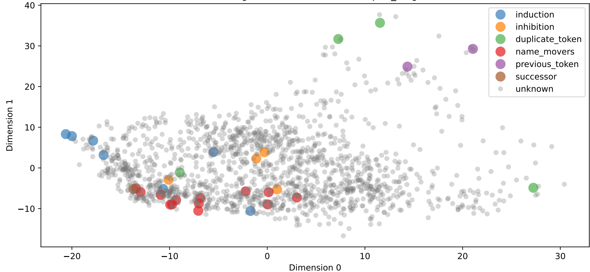
head embeddings of all models via Isomap, n_neighbors=16
