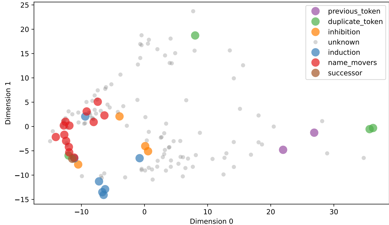
`gpt2-small` head embeddings via Isomap, n_neighbors=16
