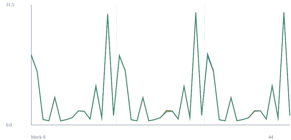
gamma = (0, 0.01)
