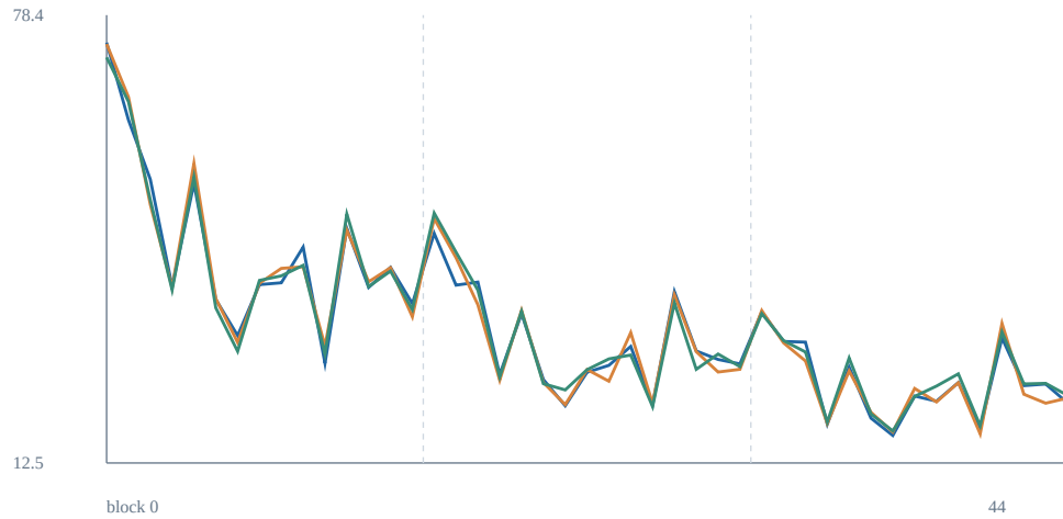
gamma = (0, 0.001)
