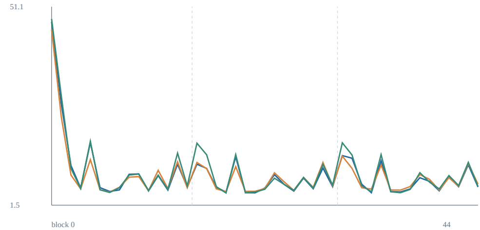
gamma = (0, 0.01)
