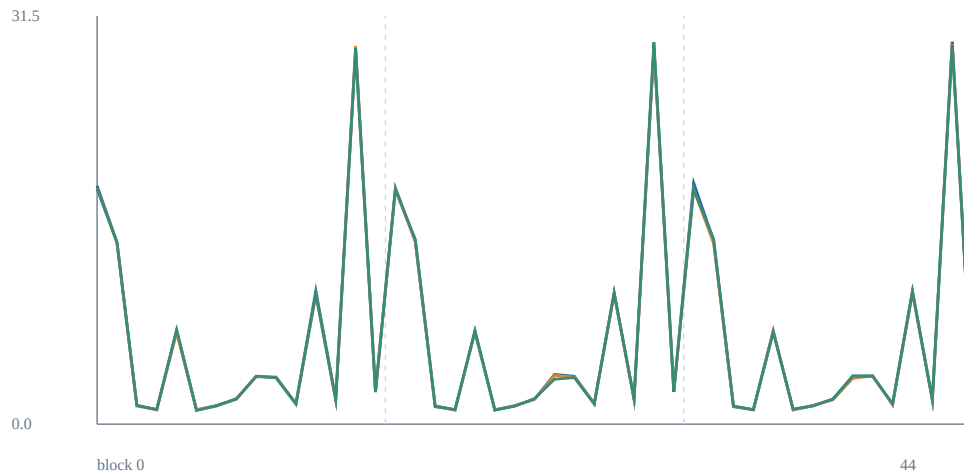
gamma = (0, 0.001)
