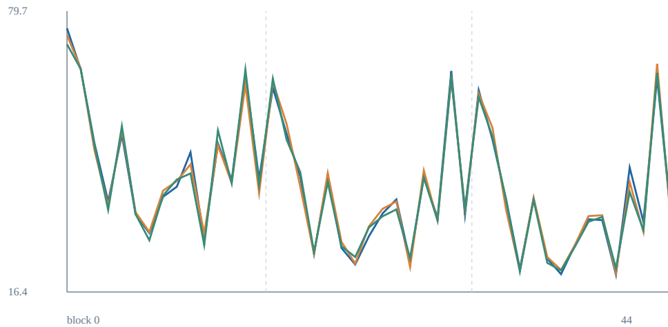
gamma = (0, 0.001)
