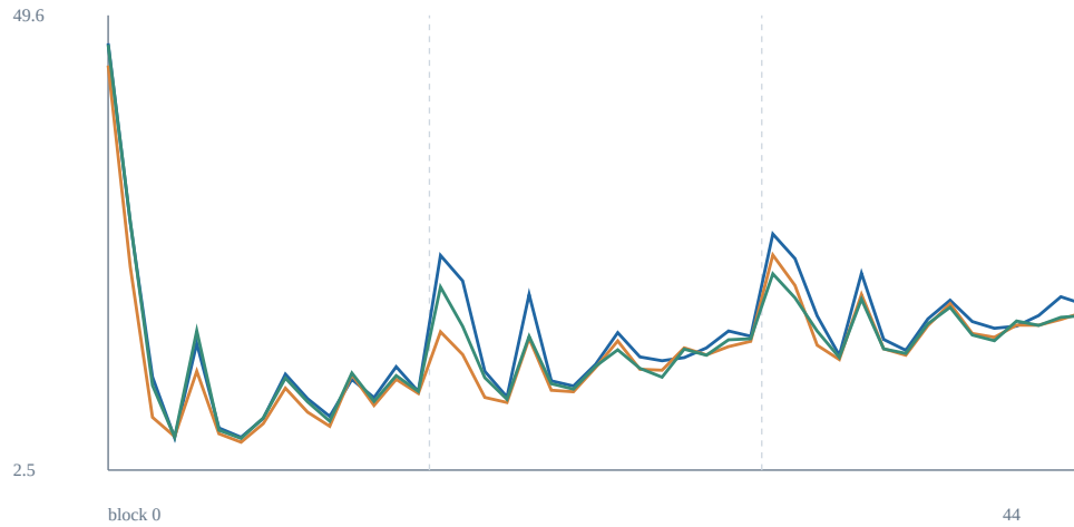
gamma = (0, 0.001)
