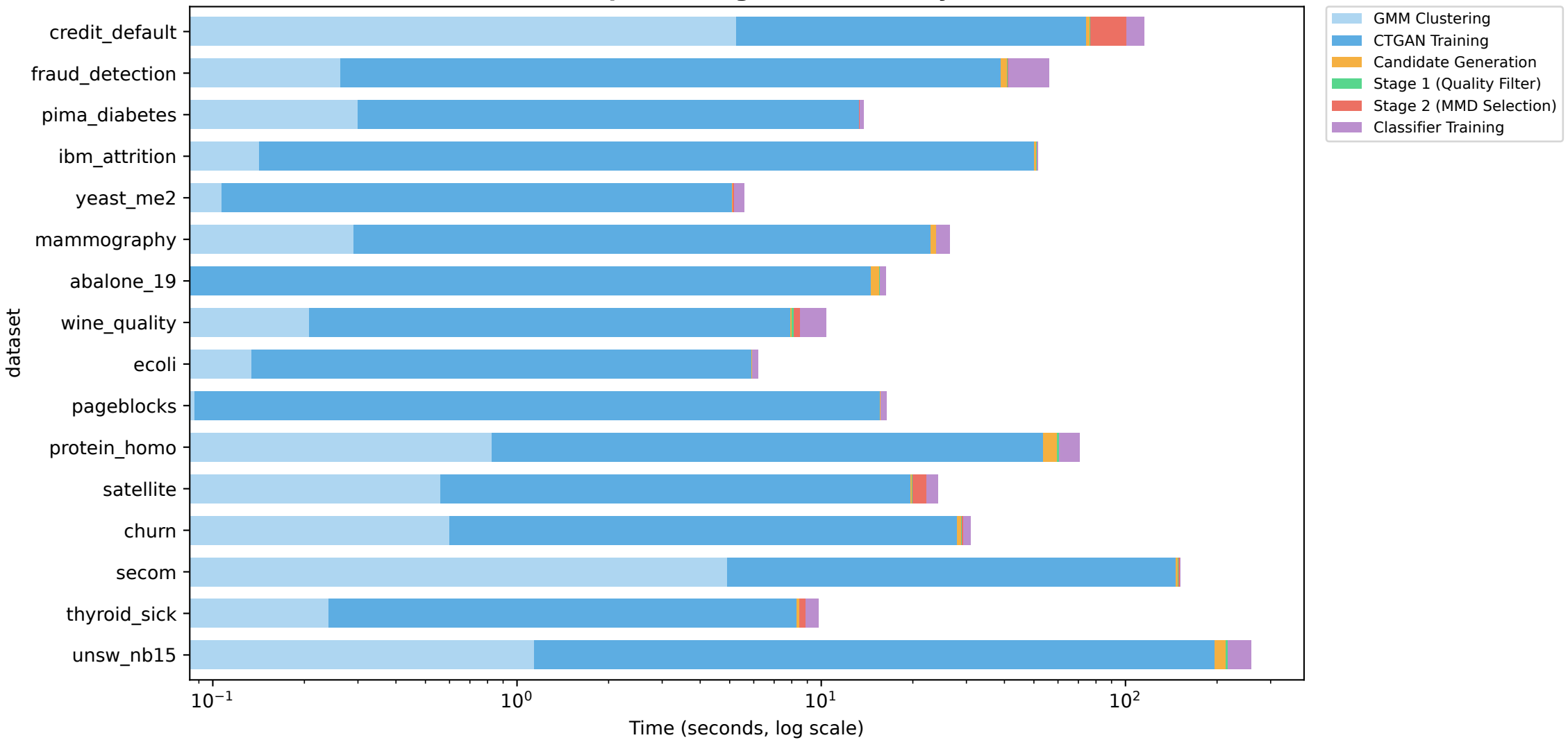
Q-G-CTGAN Pipeline Stage Breakdown by Dataset
