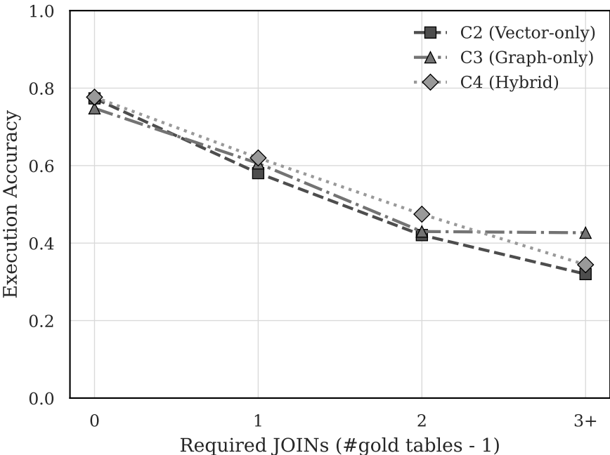
All datasets
