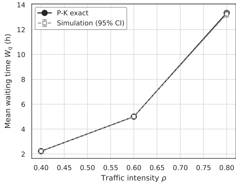
M/G/1 (exact, c = 1 )
