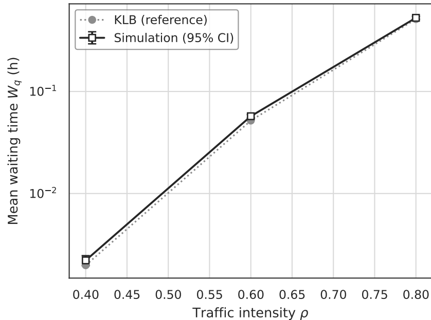
M/G/c ( c = 12 )
