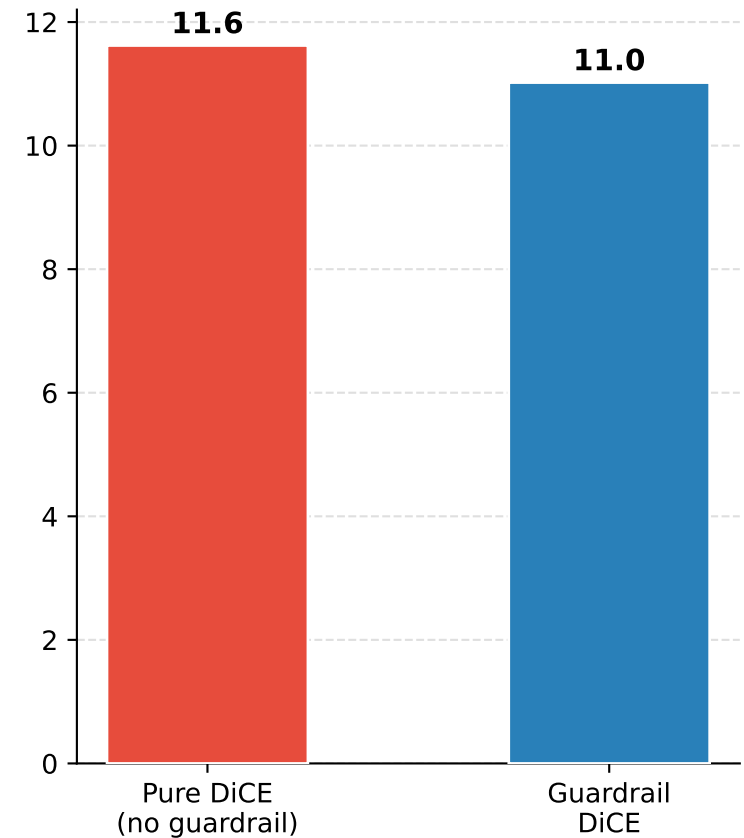
Avg. Changed Variables (Recourse Sparsity)
