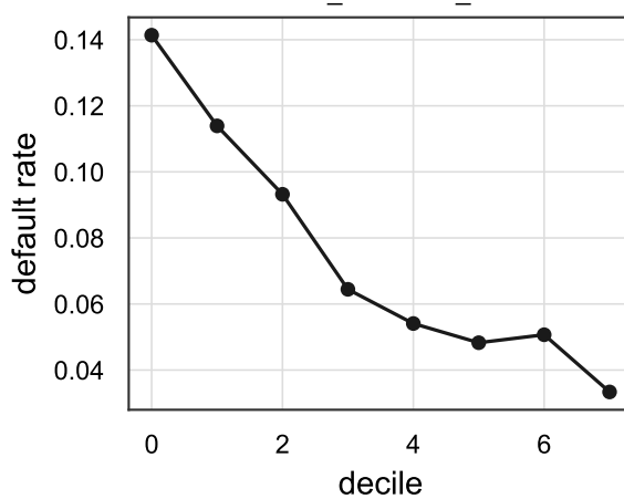
EXT_SOURCE_1
