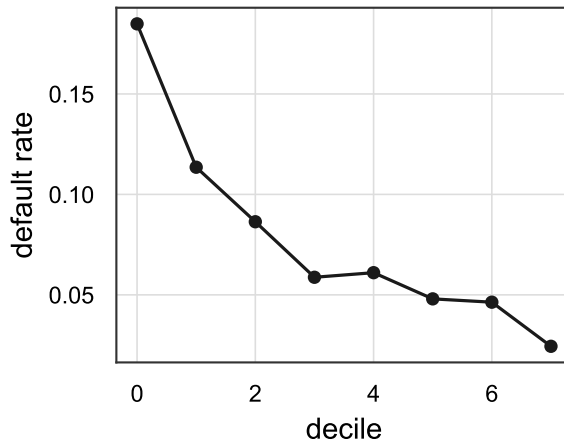
EXT_SOURCE_1
