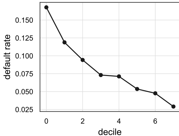
DAYS_BIRTH
