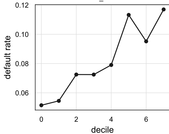
DAYS_BIRTH
