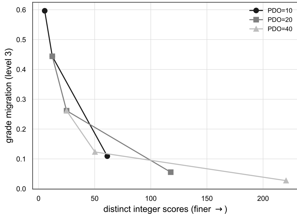
Pareto 2: quantization (deployment round())
