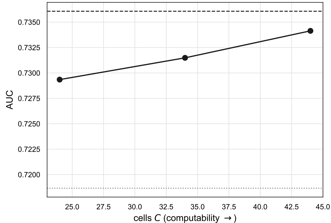
Pareto 1: approximation (price of interpretability)
