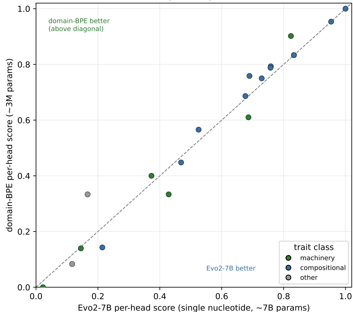
Per-trait: a tiny domain-BPE model vs a 7B genome model (species split)
