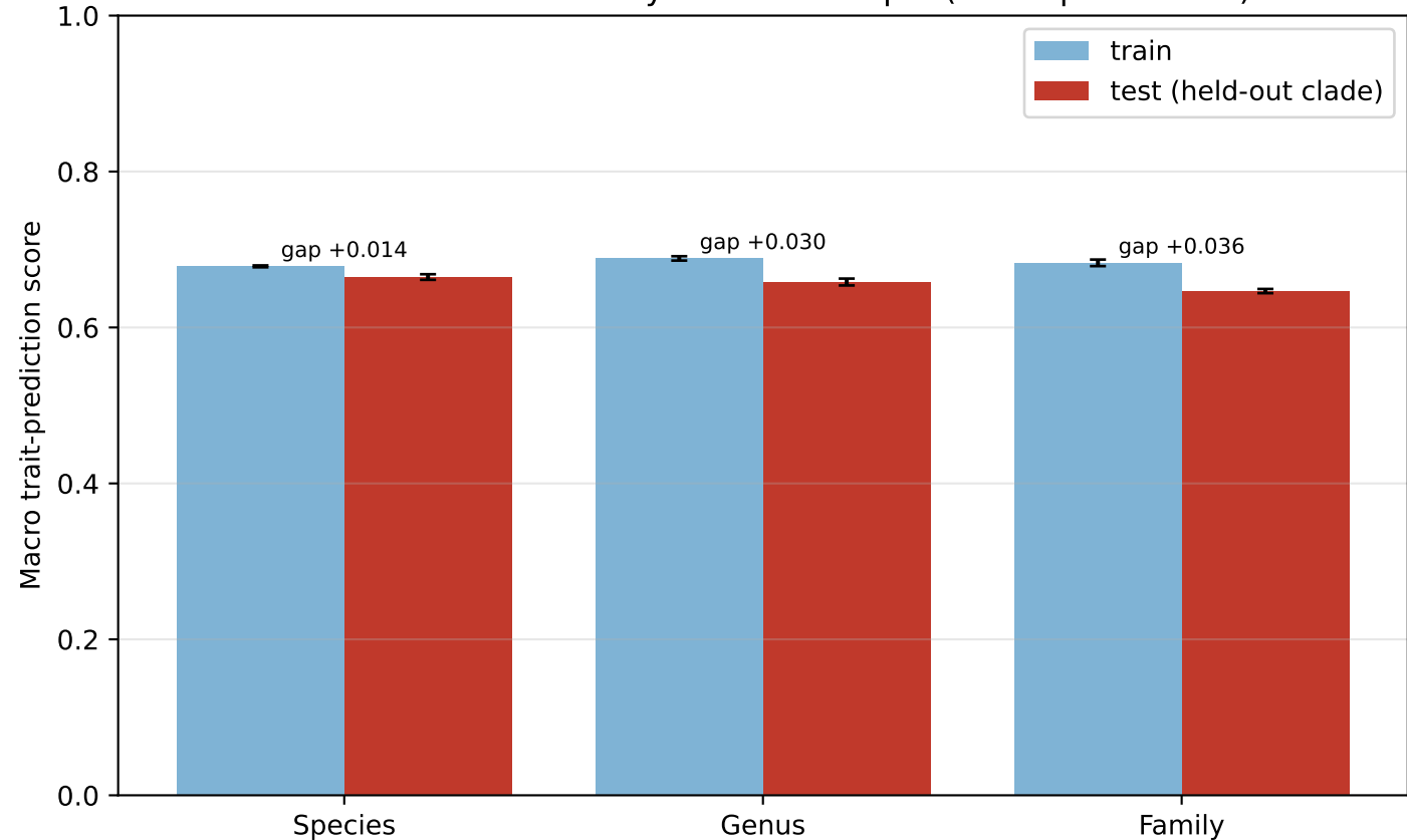
Train vs held-out test by cross-clade split (mean-pool ESM-2)
