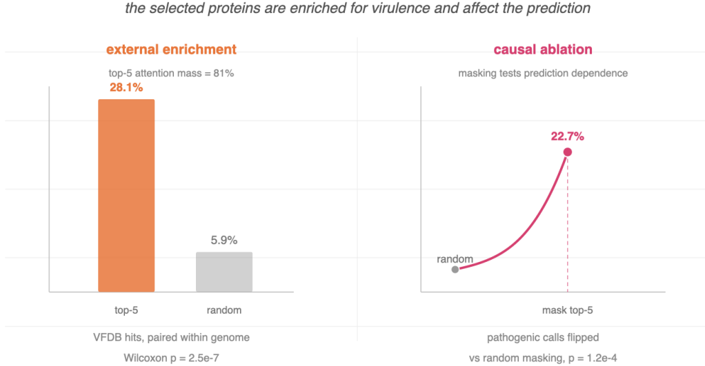
Figure 4: Mechanistic validation path. The pathogenicity result is evaluated by external database enrichment and by perturbing the selected proteins.
