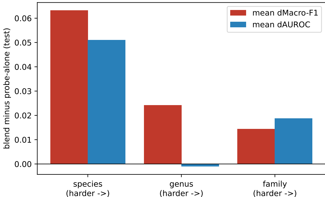
Retrieval-augmented head: marginal gain vs taxonomic distance
