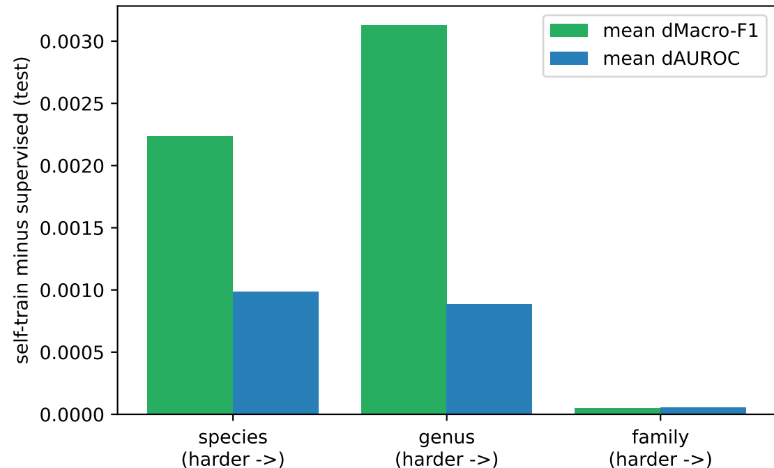
Semi-supervised self-training: gain vs taxonomic distance
