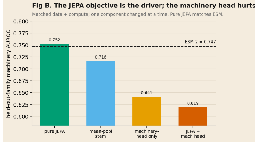
Figure 4: The self-supervised JEPA objective alone matches ESM-2; adding a genome-level machinery head hurts.
