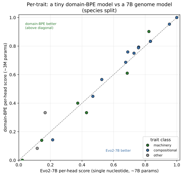
Figure 8: Per-trait, species split: a \sim 3\text{M} -parameter domain-BPE model ( y ) versus the 7B single-nucleotide Evo2 ( x ). Most heads sit on or above the diagonal: tokenization buys with 3M params what scale does not buy Evo2 with 7B.
