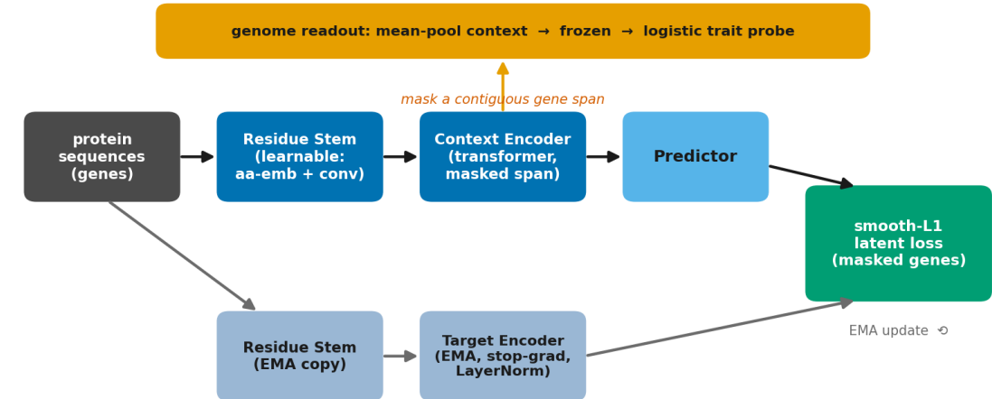
Fig A. From-scratch genome-JEPA architecture
