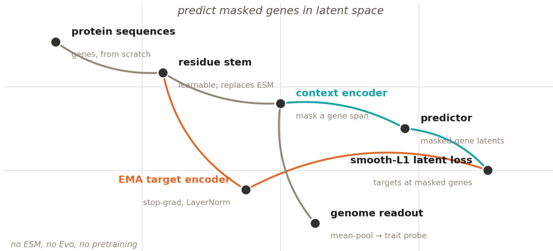
Figure 3: From-scratch genome-JEPA. A learnable residue stem feeds a context encoder whose masked-gene latents are predicted against an EMA target (smooth-L1); the pooled context is frozen and read out with a logistic trait probe. No ESM, no Evo, no pretraining.
